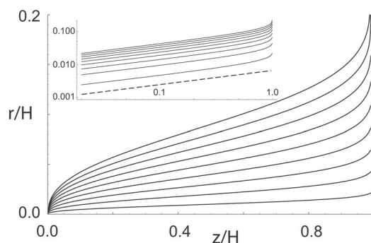
FIG. 7. Plots of the constant- \omega lines as calculated numerically in the small \theta approximations (33) for q=1.5 , giving an exponent \alpha = 1/(1+q)=0.4 close to the bottom. The inserted graph depicts the same curves on a log-log scale, and with the 0.4 power indicated by the dashed line.
