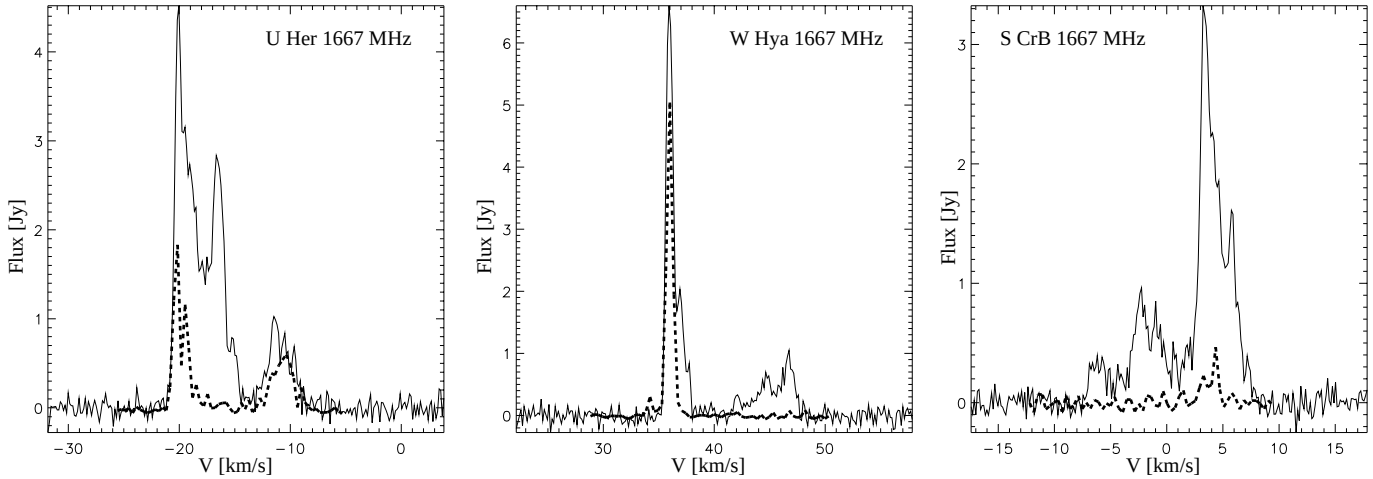
Fig. 5. The 1667 MHz maser spectra of U Her, W Hya and S CrB. The solid line is the single dish spectrum in left-hand circular polarization for U Her and S CrB and right-hand circular polarization for W Hya. The spectra are from Etoke & Le Squeren (2000) and Etoke et al. (2001), and were taken in 1984 (U Her) and 1986 (W Hya and S CrB) at the Nancay radio telescope. The thick dashed line is the maser spectrum at a short VLBA baseline (Pt-La) from the last observing epoch (May 12, 2002).
