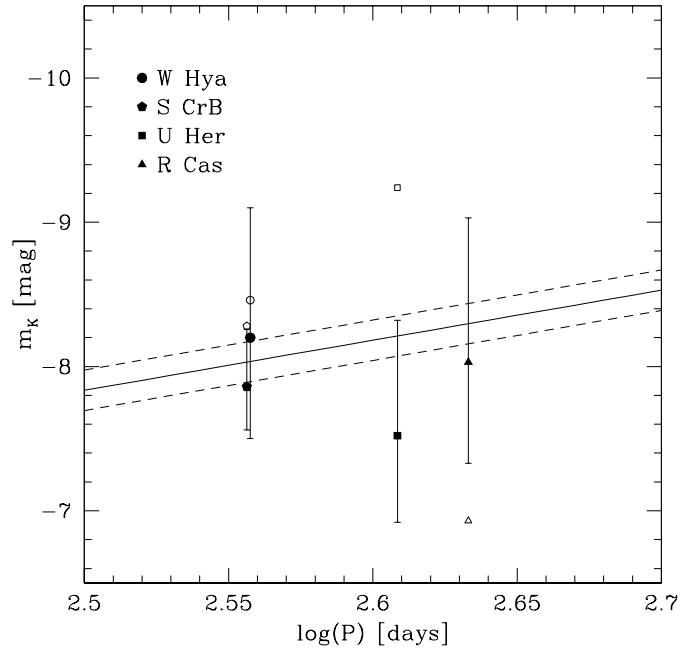
Fig. 12. Period vs. K_0 luminosity for the observed stars. The solid symbols and the error bars are determined using the distances obtained in this paper. The open symbols are the values using the Hipparcos distances. The solid line is the P – L relation determined by Whitelock & Feast (2000) on the oxygen rich Mira stars observed with Hipparcos, the dashed lines are the spread in the relation due to the error in the P – L relation zero-point.
