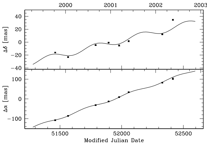
Fig. 9. Similar to Fig. 6. The position of the brightest 1665 MHz maser spot of R Cas with respect to J2355+495. The brightest R Cas maser feature is red-shifted with respect to the stellar velocity. Drawn is the best fitting parallax and proper motion trajectory combining the results on both maser transitions for the 8 epochs of observations.
