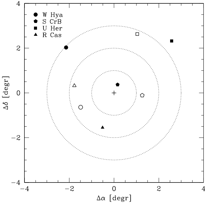
Fig. 1. Reference source positions wrt the target star in Right Ascension and Declination off-set. The sources are indicated with the listed symbols where the solid symbols are reference source 1, and the open symbols reference source 2. The circles are plotted to guide the eye and have a diameter of 2, 4 and 6 degrees.
