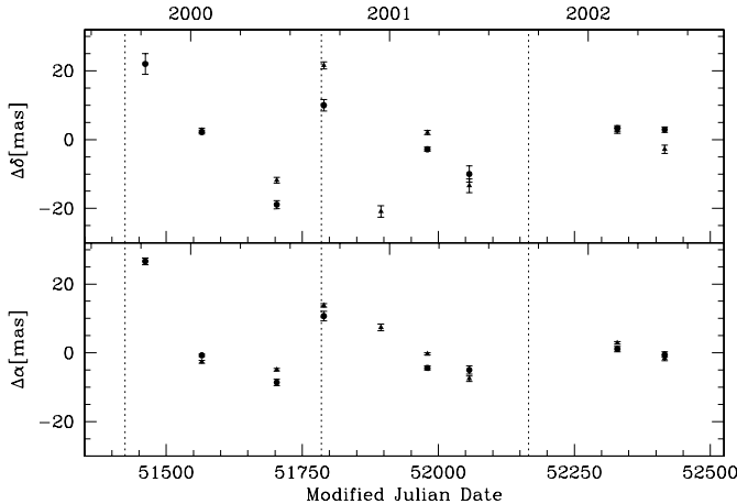
Fig. 11. The residual motion of the maser spots of W Hya after subtracting the best fitted model. The circles are the 1667 MHz spot and the triangles the 1665 MHz spot. The errors are the formal position fitting errors. The dashed vertical lines indicate the position of the maximum of the stellar phase.
