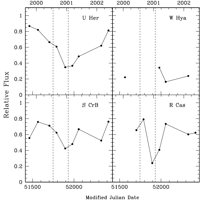
Fig. 2. The ratio between the flux density of reference source 1 when phase-referenced to reference source 2 and the flux density when using the phase, delay and phase rate solutions obtained on reference source 1 itself. The dashed vertical lines indicates the approximate period maximum solar activity.
