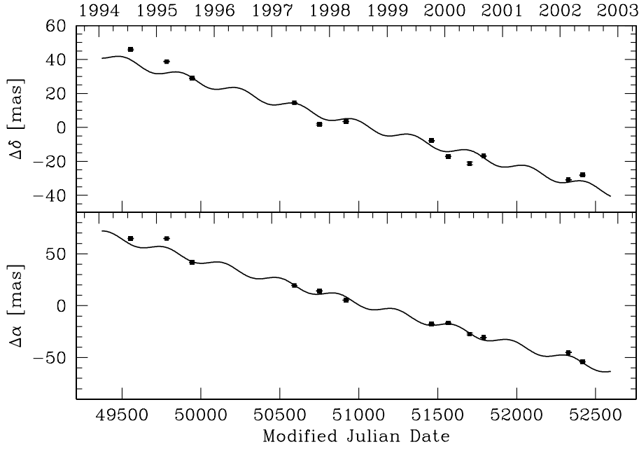
Fig. 6. The position of the most blue-shifted 1667 MHz maser spot of U Her with respect to J1630+2131. The error bars on the positions indicate the formal position fitting errors. The solid line is the best fitting parallax and proper motion trajectory for the 12 epochs of observations. Note that the scales are different for declination and right ascension.
