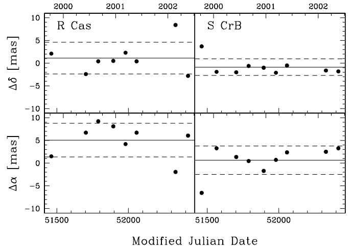
Fig. 4. The difference between the measured separation and its a priori value of S CrB reference source 1 (J1522+3144) with respect to 2 (J1527+3115), and R Cas reference source 2 (J2347+5142) with respect to 1 (J2355+495). The formal error bars lie within the plotted symbols. The solid line indicates the average separation between the reference sources and the dashed lines are the rms.
