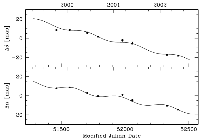
Fig. 8. Similar to Fig. 6. The position of the brightest 1665 and 1667 MHz maser spots of S CrB with respect to J1522+3144. The brightest S CrB maser feature is red-shifted with respect to the stellar velocity. The 1665 and 1667 maser spots have the same velocity. Drawn is the best fitting parallax and proper motion trajectory combining the results on both maser transitions for the 8 epochs of observations.
