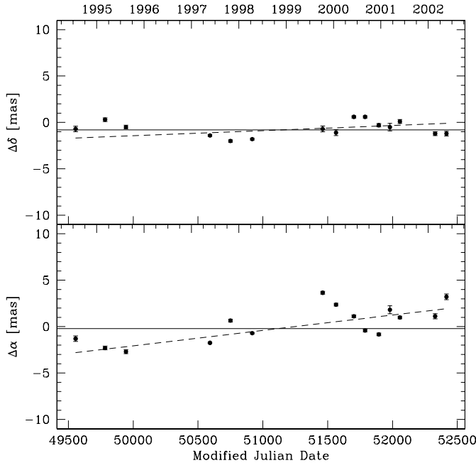
Fig. 3. The difference between the measured separation and its a priori value of U Her reference source 1 (J1636+2112) with respect to 2 (J1630+2131, formerly J1628+214). The solid line indicates the average separation between the reference sources. The dashed line is a weighted least square fit to a change in measured separation due to evolving source structure of J1630+2131.
