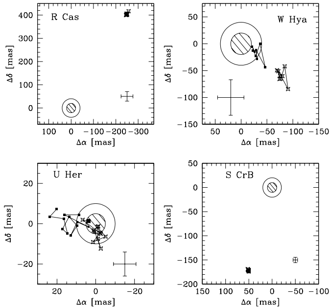
Fig. 10. The position of the observed maser spot wrt the optical position as predicted by our fits. The solid symbols denote the first epoch and subsequent epochs are connected. Also drawn are indications of the size of the star (shaded) and the radiophotosphere. The error bars in the corner are the errors due to the transposition of the radio positions and the Hipparcos position errors. The exact size of the error bars depends on the epoch of observations, the drawn error bars are for the middle epoch. For U Her and W Hya the squares indicate the transposed positions using the Hipparcos proper motion and parallax. Note the difference in scale of the four plots.
