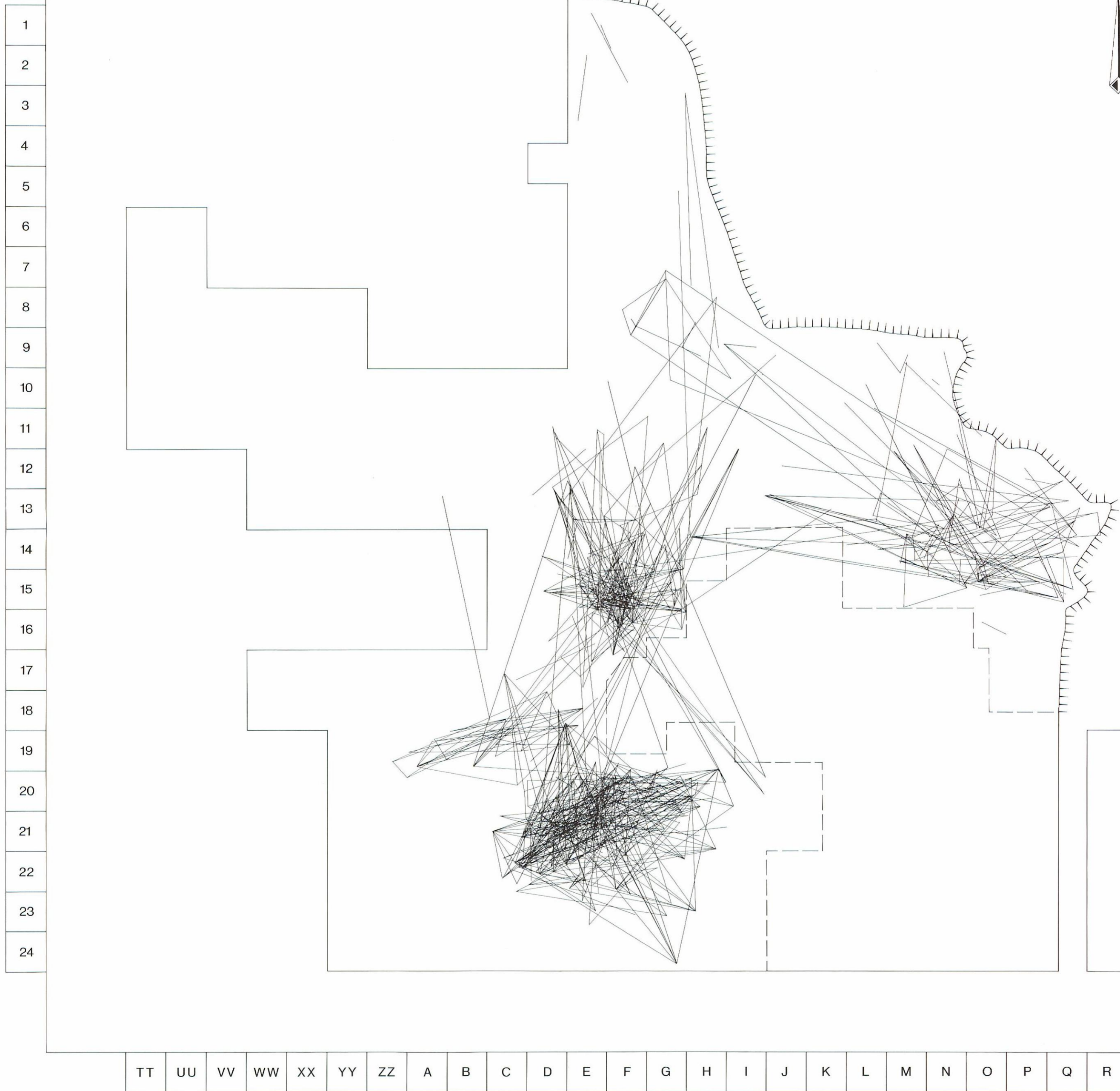
Fig. 47. Maastricht-Belvédère, Site C. Horizontal distribution of all refitted artefacts, each line representing the liaison between two refitted artefacts (see figure 45, model C). Scale 1:80 (Reference grid in square metres).
