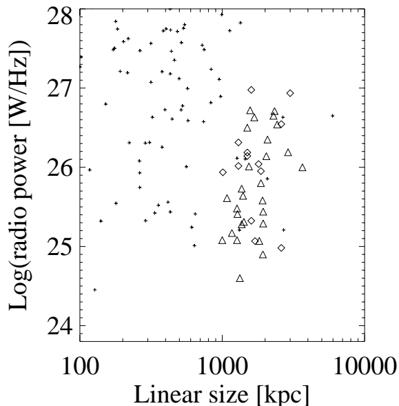
Fig. 3. The 325-MHz radio power against linear size P – D diagram for the formerly known GRGs not part of the LRL sample (diamonds), the newly discovered GRGs (triangles) and sources from the LRL sample with z < 0.6 (plusses).
