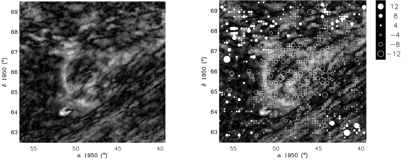
Fig. 2. P and RM for the region in the constellation of Horologium centered at (l, b) = (137^\circ, 7^\circ) . Notation as in Fig. 1, where the maximum P = 95 mJy/beam corresponds to T_{b,pol} = 13.9 K.
