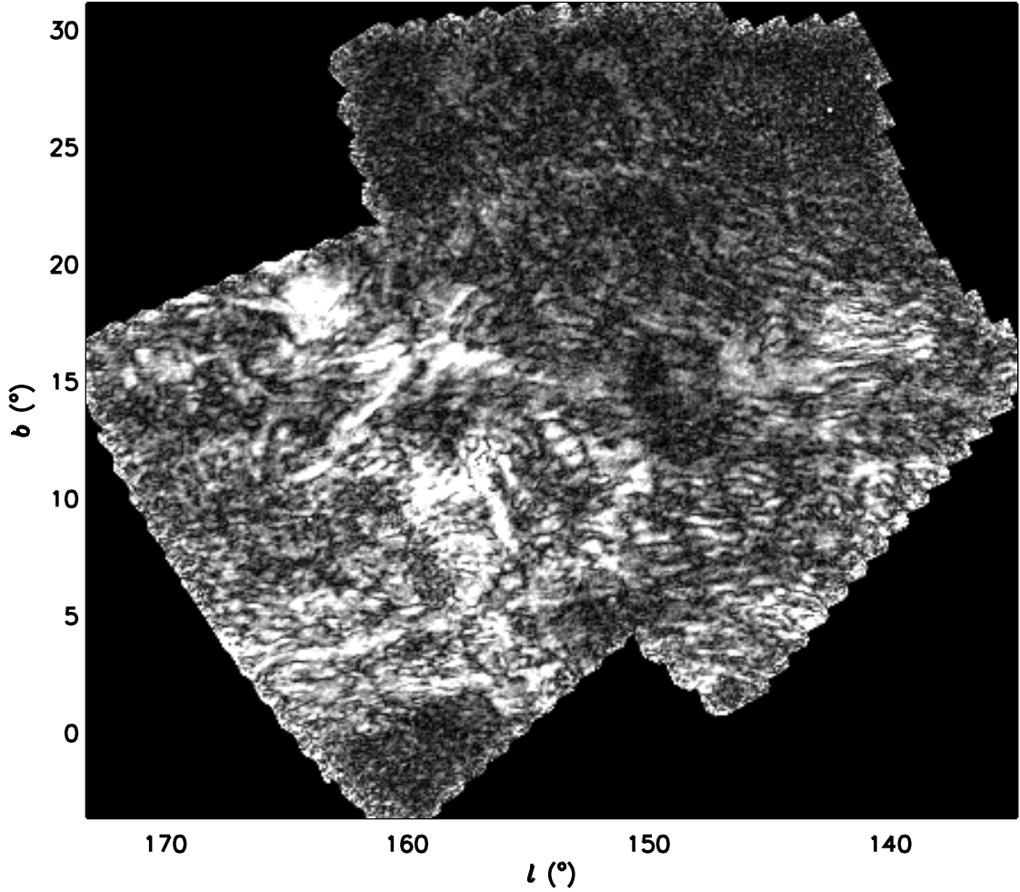
Fig. 3. Grey scale representation of the polarized intensity of the polarization part of the WENSS survey at 325 MHz, where white denotes a maximum intensity of 35 mJy/beam ( T_{b,\text{pol}} \approx 17 K to 25 K, depending on declination). The data were smoothed with a 500m taper, and have a resolution of \sim 2.5' .
