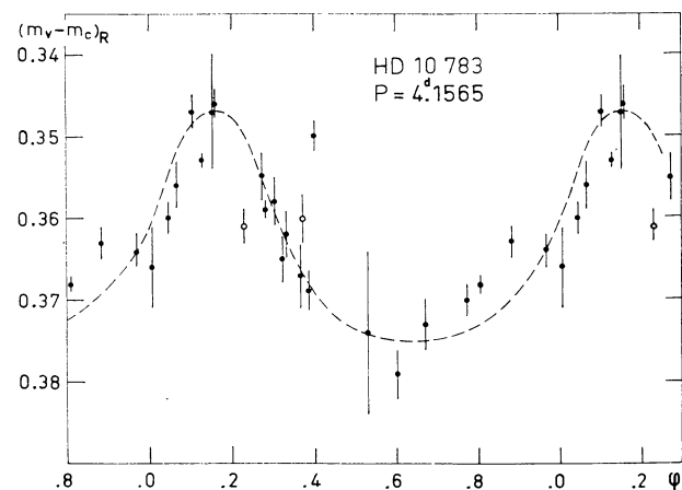
Figure 2. The light-curve of HD 10783 in red light ( \lambda_{\text{eff}} = 5960 Å). The mean errors are indicated by lines. Open circles are the mean values of less than five observations.
