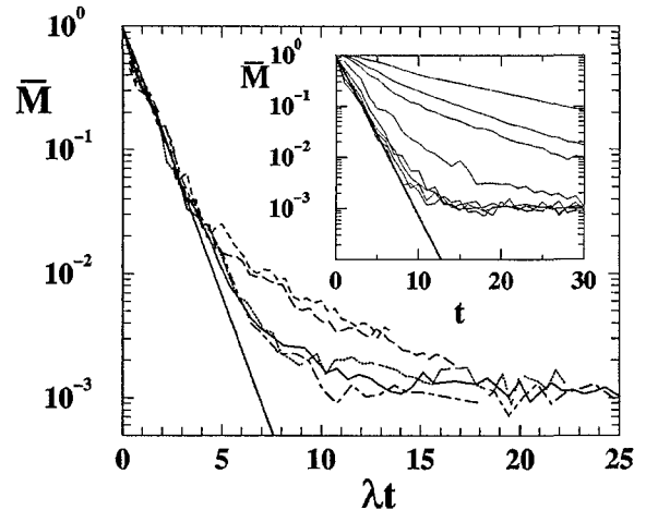
FIG 4 Decay of \bar{M} in the Lyapunov regime, for \phi = 2.1 \times 10^{-3} , K=2.7, 3.3, 3.6, 3.9, 4.2 . The time is rescaled with the Lyapunov exponent \lambda , ranging from 0.22 – 0.72 . The straight solid line indicates the decay \bar{M} \propto \exp(-\lambda t) . Inset: \bar{M} for K=4.2 and different \phi=j \times 10^{-4} , j=1, 2, 3, 4, 5, 9, 17, 25 . The decay slope saturates at the value \phi \approx 1.7 \times 10^{-3} for which \Gamma \approx \lambda , even though \Gamma keeps on increasing. This demonstrates the decay law \bar{M} \propto \exp(-\gamma t) with \gamma = \min(\Gamma, \lambda) .
