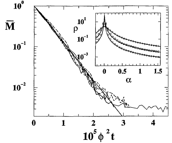
FIG 2 Decay of \bar{M} in the golden rule regime for kicking strengths K=13.1, 17.1 , and 21.1 as a function of the rescaled time \phi^2 t . Perturbation strengths range from \phi=10^{-4} to 10^{-3} . Inset: Local spectral density of states for K=13.1 and perturbation strengths \phi=2.5 \times 10^{-4}, 5 \times 10^{-4}, 10^{-3} . The solid curves are Lorentzian fits, from which the decay rate \Gamma \approx 0.84 \phi^2 S^2 is extracted. The solid line in the main plot gives the decay \bar{M} \propto \exp(-\Gamma t) with this value of \Gamma .
