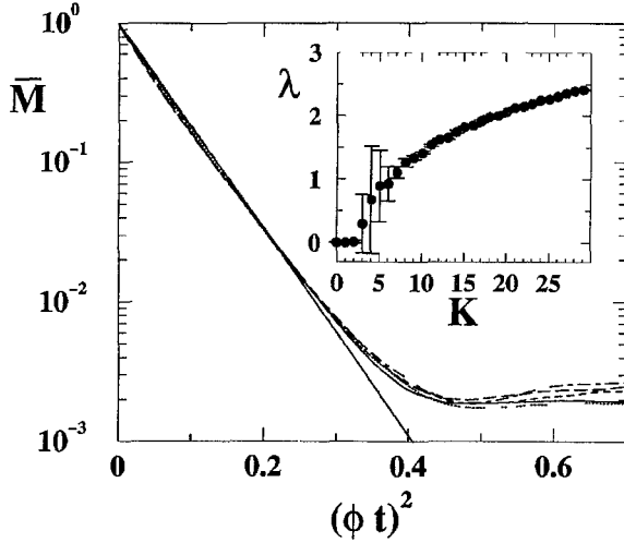
FIG 1 Decay of the average fidelity \bar{M} for the quantum kicked top with K=13.1 and S=500 , as a function of the squared rescaled time (\phi t)^2 . The perturbation strengths range between \phi=10^{-7} and 10^{-6} . The straight line corresponds to the Gaussian decay (6) valid in the perturbative regime. Inset: Numerically computed Lyapunov exponent for the classical kicked top as a function of the kicking strength K . Dots correspond to averages taken over 10^4 initial conditions (see Ref. [10]). The error bars reflect different results obtained with different initial conditions. The vanishing of error bars indicates the disappearance of islands of regular dynamics.
