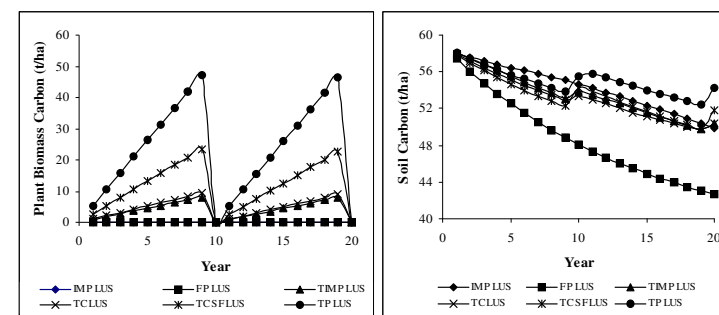
Figure 4: Predicted carbon stocks in above-ground biomass and soil (t/ha) over time of alternative land use systems, Claveria, Misamis Oriental, Philippines
