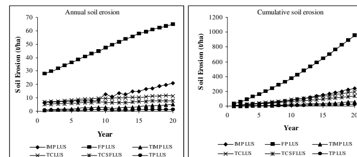
Figure 3: Predicted annual and cumulative soil erosion (t/ha) over time of alternative land use systems, Claveria, Misamis Oriental, Philippines
