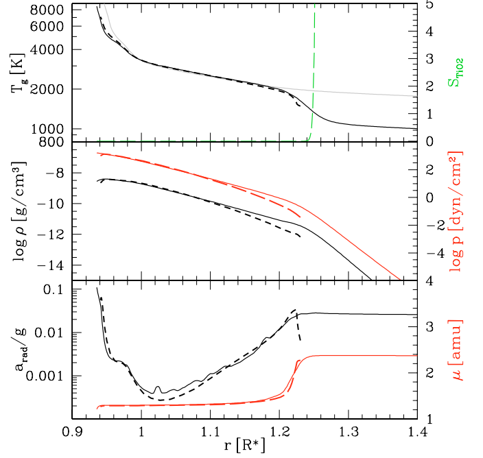
Fig. 2. Hydrostatic initial model (full) in comparison to a spherical MARCS model (dashed) and a grey model (grey T_g -line) for M_\star = 1 M_\odot , T_\star = 2800 \text{ K} , \log g = -0.6 ( L_\star = 6048 L_\odot ), Z = 1 . S_{\text{TiO}_2} shows the supersaturation ratio of \text{TiO}_2 , indicating that nucleation is already possible very close to the star. Long-dashed graphs belong to the r.h.s. axis.
