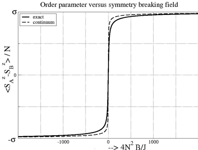
FIG. 3. Order parameter as a function of symmetry breaking field. The exact result for N=100 spins, the continuum expression for the order parameter is derived in the Appendix.
