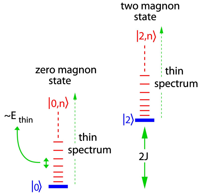
FIG. 4. (Color online) Energy level scheme with the zero and two magnon states, each with its tower of thin spectrum states. The level spacing in the thin spectrum is E_{thin} , magnons live on an energy scale J .
