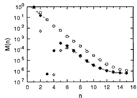
FIG. 1. The overlap M at t=n for the quantum kicked rotator for three different ways of averaging: \circ \bar{M} , \diamond \exp(-\exp(\ln(-\ln M))) , \bullet \exp(-\exp(\ln(-\ln M))) . We took K=10 , \delta K=1.6 \times 10^{-3} , N=10^6 . Averages are taken over 2000 random initial conditions of a Gaussian wave packet. The dotted line shows the Lyapunov decay \propto e^{-n\lambda_1} with \lambda_1=1.1 . At n=3 , we have only an upper bound for the logarithmic averages because cancellations in the calculation limit the accuracy.
