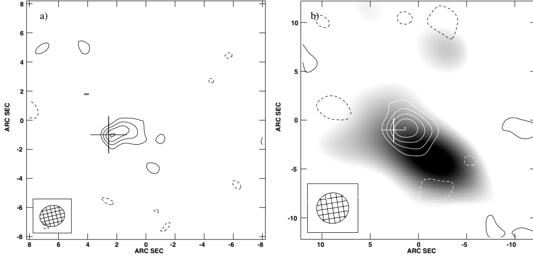
Fig. 5. a) Naturally weighted CO J = 1-0 map of the broad component obtained by combining the entire data-set and tapering it with a Gaussian with a half-width at 0.30 amplitude of 200\text{ k}\lambda . The spatial resolution is 1''.72 \times 1''.45 with the major axis PA = 283^\circ . The contours are at -2, 2, 3, 4 , and 5 \times \sigma , where \sigma = 35\text{ }\mu\text{Jy beam}^{-1} . b) The CO J = 1-0 emission tapered down to 60\text{ k}\lambda ( FWHM = 3''.33 \times 3''.12 ) overlaid as contours on a gray-scale representation of the J = 4-3 emission by Papadopoulos et al. (2000). The contours are -2, 2, 3, 4, 5 , and 6\sigma with \sigma = 0.4\text{ mJy beam}^{-1} , and the gray-scale range is 0.6-2.0\text{ mJy beam}^{-1} .
