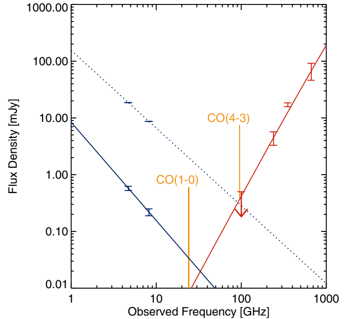
Fig. 2. The submm/far-IR spectral energy distribution (SED) of 4C 60.07 (red line) along with the radio spectra of the A-component (blue dotted line) and the radio core (blue solid line). The submm points are taken from SCUBA observations by Archibald et al. (2001) while the IRAM 30 m Telescope data-points at 252 GHz (1.25 mm) and 100 GHz (3 mm) are from Papadopoulos et al. (2000). The radio points are measured from C and X band data of 4C 60.07 from the VLA Archive. The positions and strengths of the CO J = 1-0 and J = 4-3 lines relative to the SED are shown in yellow (based on this paper and Papadopoulos et al. 2000).
