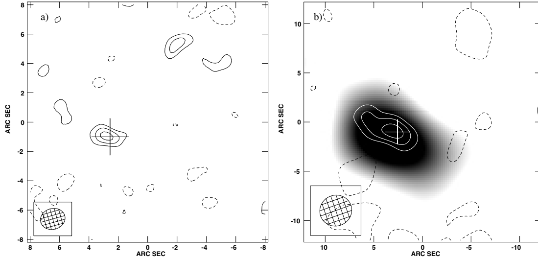
Fig. 7. a) The narrow component tapered at 200 kλ. The resolution is 1''.72 \times 1''.42 at PA = 285^\circ . Contours are at -2, 2, 3 , and 4 \times \sigma , where \sigma = 55 \mu\text{Jy beam}^{-1} . b) The CO J = 1-0 emission tapered down to 60 kλ ( \text{FWHM} = 3''.22 \times 3''.07 ) overlaid as contours on a gray-scale representation of the J = 4-3 detection by Papadopoulos et al. (2000). The contours are -2, 2, 3 , and 4\sigma with \sigma = 0.6 \text{ mJy beam}^{-1} , and the gray-scale range is 0.6-2.0 \text{ mJy beam}^{-1} .
