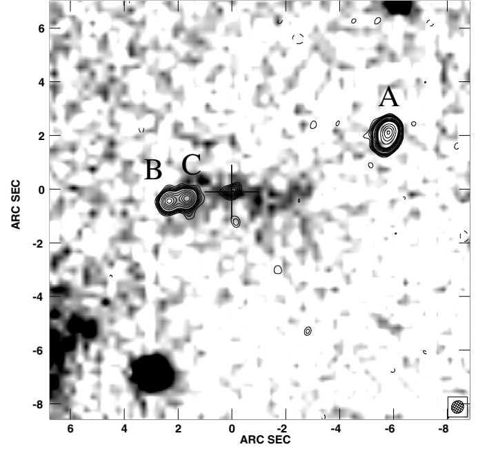
Fig. 1. 6 cm VLA map of 4C 60.07 overlaid on an I -band image obtained with the William Herschel Telescope. The radio hot spots are denoted by A, B and C. The cross marks the position of the radio core: RA(J2000): 05^{\text{h}}12^{\text{m}}55^{\text{s}}.147 , Dec(J2000): +60^{\circ}30'51''.0 . The insert in the bottom right corner shows the synthesized beam.
