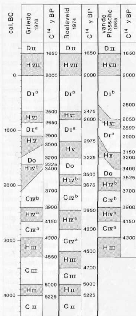
Figure 5 Chronological-stratigraphical division of the Holocene in the northern Netherlands. After Griede 1978 and Van de Plassche 1985.
