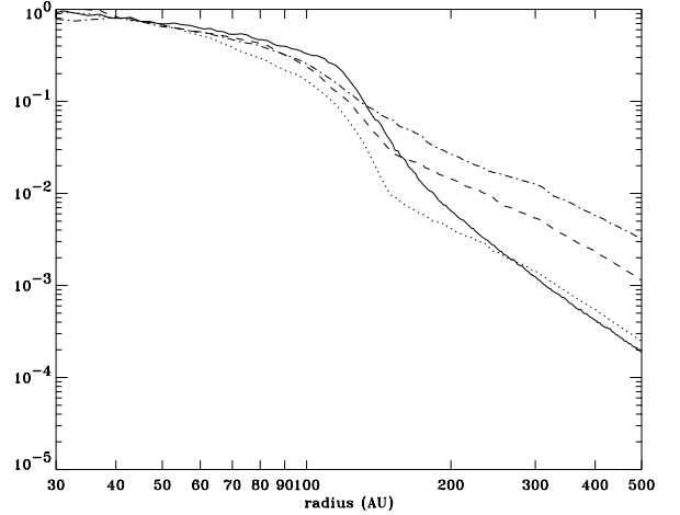
Fig. 6. Profiles obtained for different dust size distributions in the high gas density disc (case 1). dash-dot line: dN \propto s^{-3.5} ds , dashed line: dN \propto s^{-3} ds , dotted line: dN \propto s^{-2.5} ds . The solid line is the reference gas-free profile of Fig. 3.
