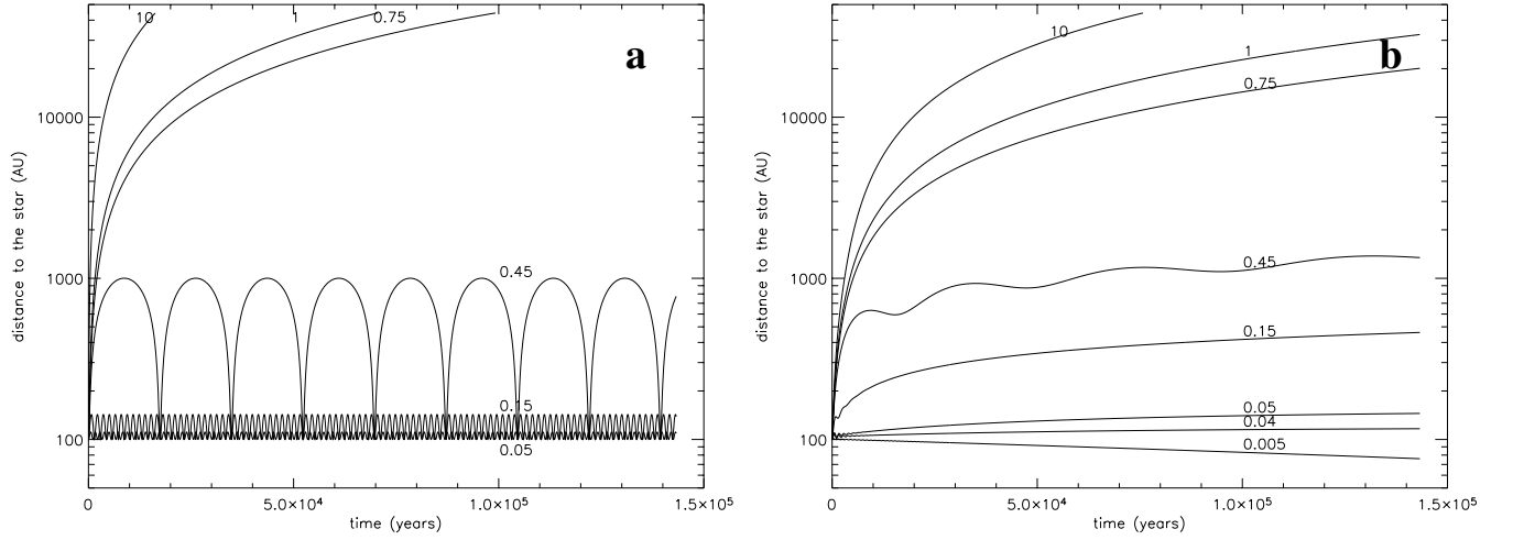
Fig. 2. Radial position as a function of time, for different values of \beta , for one particle initially located at 100 AU: a) gas-free case b) high gas density case (case 1). Note how efficient gas drag partially erases the abrupt transition at \beta = 0.5 for the dynamical behaviour of small grains.
