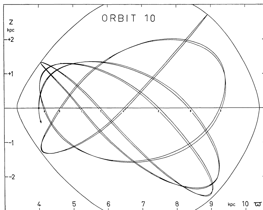
Orbit 10, low, special , frequency ratio near 14 : 17. In revolution 5 the fundamental point D is approached closely, after which the previous path is nearly retraced back to the starting point ( \varpi = \varpi_A , z = 0 ).
