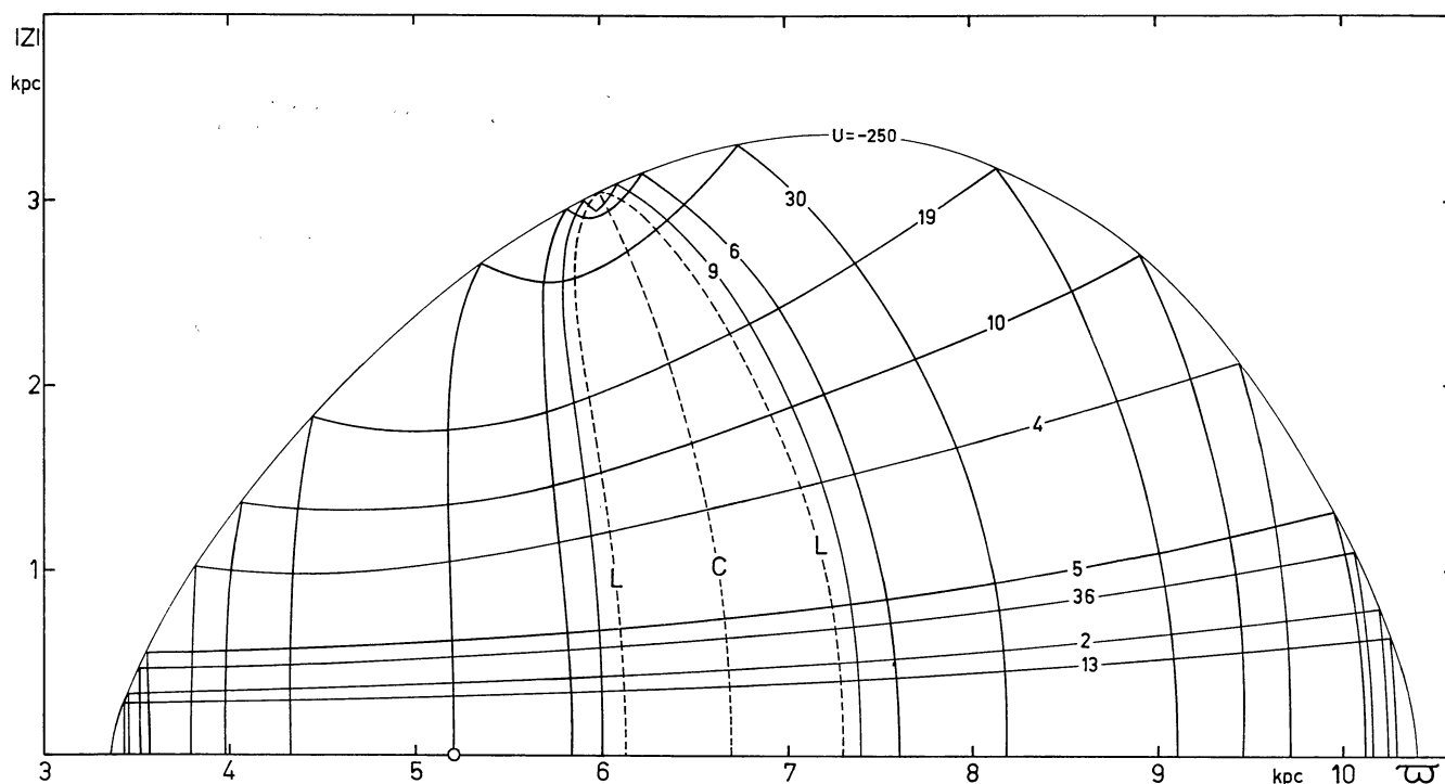
Envelopes of each of the orbits discussed in this thesis; corners of each envelope are rectangular, mutual intersections of the envelopes are not rectangular. Broken line marked L: limiting orbit. Broken line marked C: central orbit.
