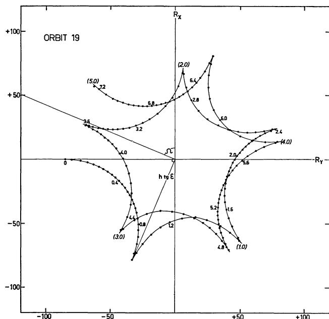
Projection of tip of angular-momentum vector on the galactic plane for orbit 19. Motion of orbital plane is retrograde. Time interval between two dots: 0.04 time units = 3.9 \cdot 10^6 years. Every 10 time intervals the dot is marked with the time in time units. Longitude of ascending node \mathcal{L}_0 can be found graphically as illustrated for the first passage through the galactic plane ( t \approx 1.0 ). Length of line section in which h \text{ tg } \epsilon is written, is equal to this quantity. Units in both coordinates: 10 \text{ km.kpc/sec} .
