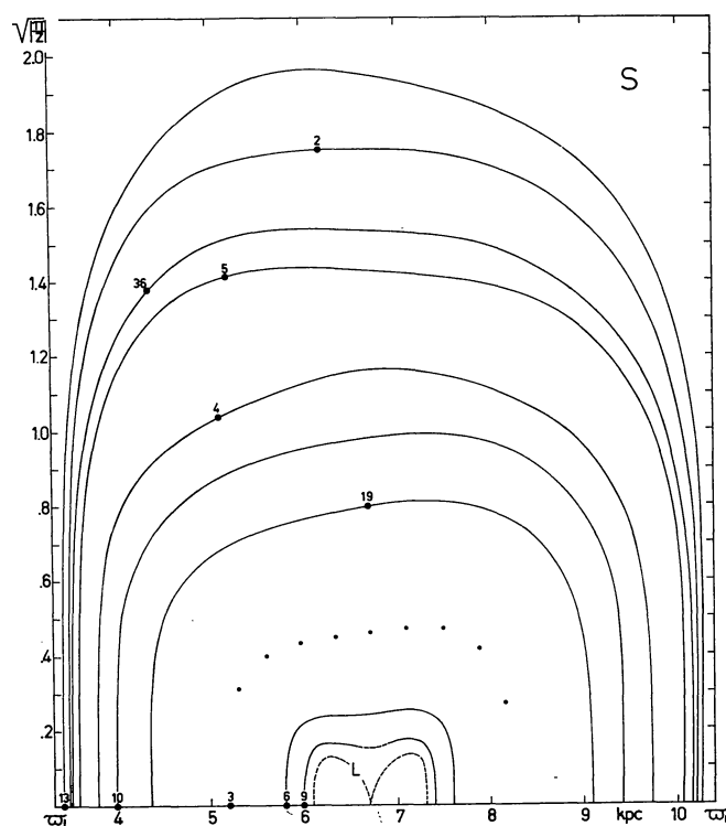
Inclination diagram for the box-type orbits. A filled circle indicates the starting point. Orbit 3 (periodic) is represented by a series of 10 points. Inclination curve of orbit 30 is not drawn but passes close to these points. For orbit 9, not computed long enough to give the entire curve, the broken line indicates the missing section. Broken lines marked L: limiting orbit.
