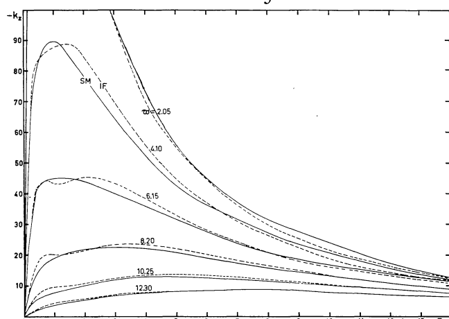
Force components perpendicular to the galactic plane at various \omega (unit 100 \text{ km}^2/\text{sec}^2.\text{kpc} ), in the SCHMIDT model and in the interpolation formula.
