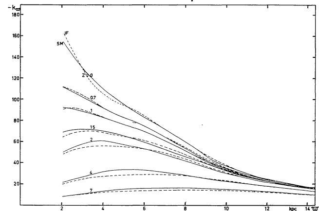
Radial force components in and outside the galactic plane (unit 100 km 2 /sec 2 .kpc), in the SCHMIDT model and in the interpolation formula.
