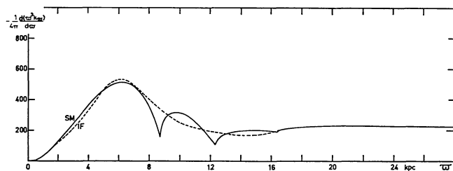
Curve demonstrating the absence of unstable circular orbits in the final SCHMIDT model and in the force function K_{\varpi} of the interpolation formula. Unit in ordinate: 100 \text{ km}^2 \cdot \text{kpc}/\text{sec}^2 .
