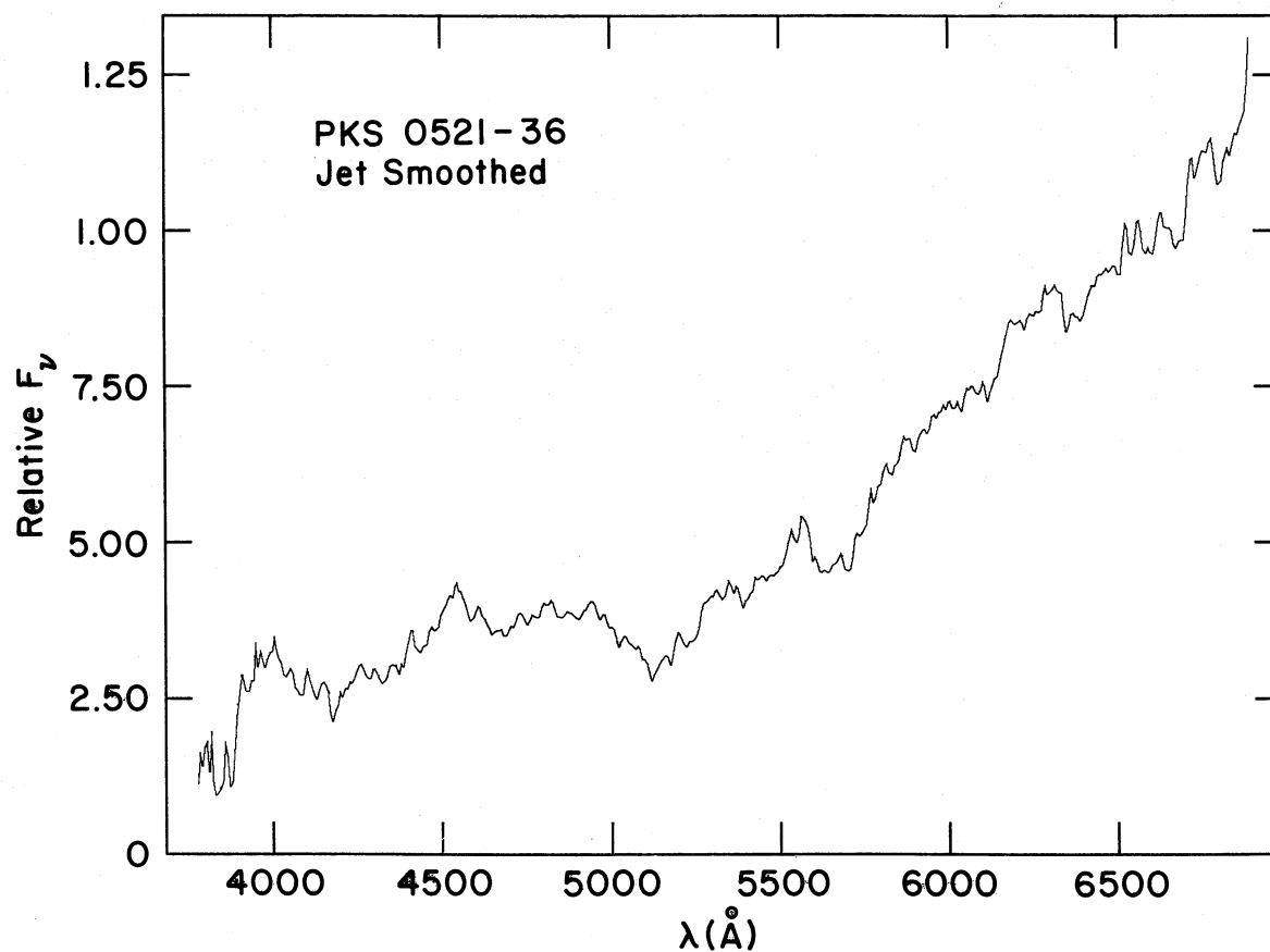
FIG. 6.—EFOSC spectrum of the jet of PKS 0521–36, smoothed with a 125 Å rectangular filter and shown as flux per unit frequency. The steep continuum matches that seen from multicolor imaging; no significant spectral features are present.
