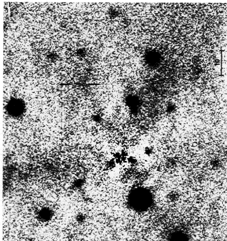
NGC 6251 (R)
