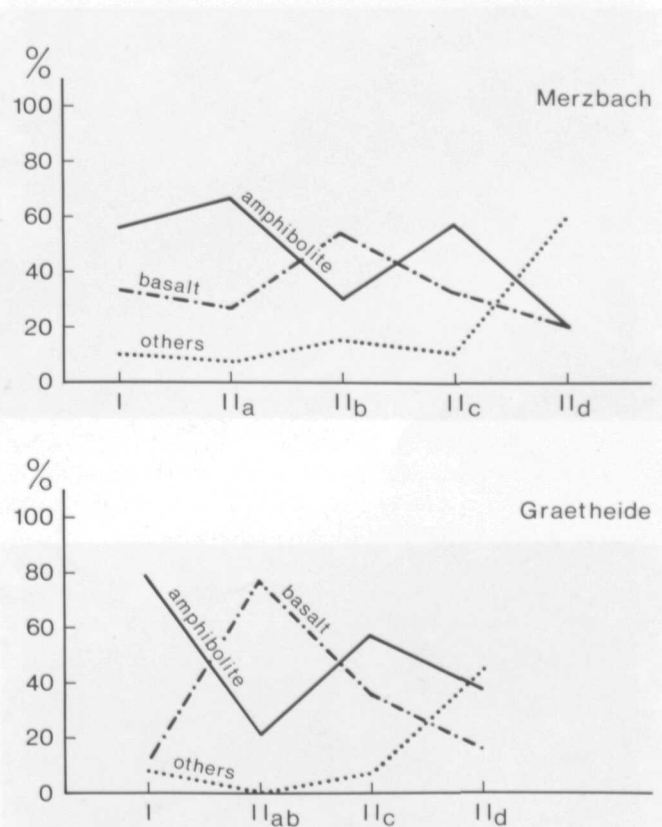
Fig. 11 The relation between rock-type and phase.
