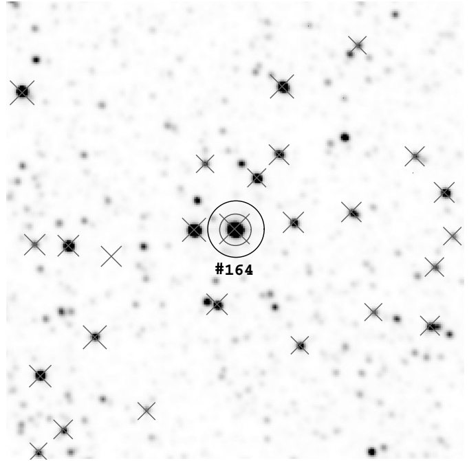
Fig. 5. 2MASS K_S image 230'' \times 230'' centred at the position of #164. The black circle delimits the main beam (FWHM) of the IRAM telescope used for the SiO maser search. A small gray circle marks the 2MASS association and finally crosses mark sources detected by ISOGAL. In agreement with the discussion in the text, all the ISOGAL and 2MASS positions are in excellent agreement. Note that the targeted source is the only mid-infrared source falling inside the IRAM telescope beam.
