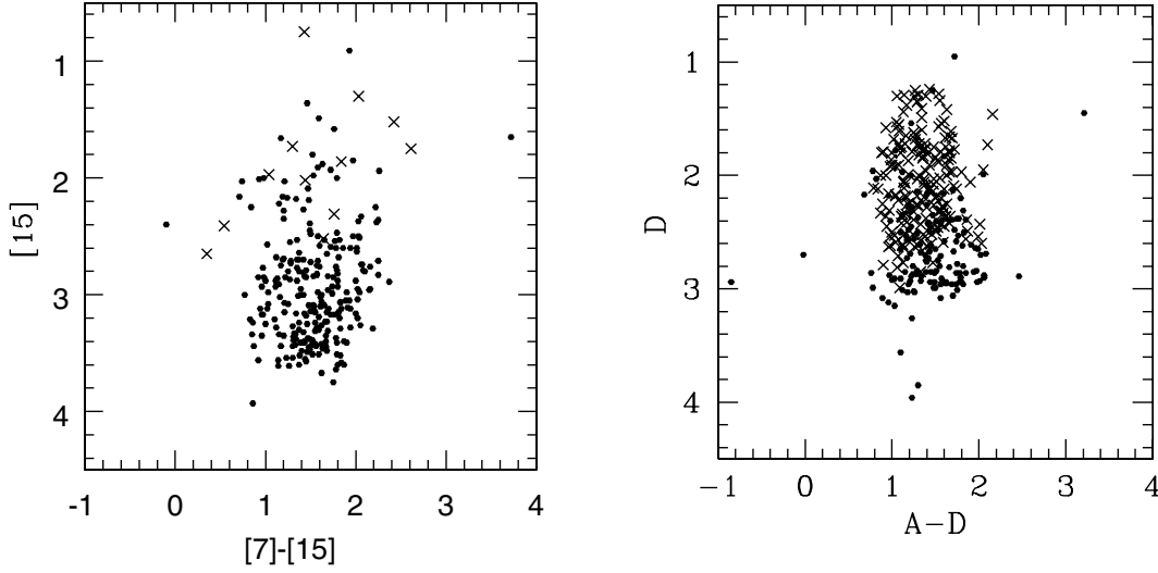
Fig. 9. Mid-infrared colour-magnitude diagrams. Left-hand panel: all data from ISO GAL. Right-hand panel: all data from MSX. Filled circles indicate targets from the ISO GAL sample and crosses indicate targets from the MSX sample. The two samples have similar mid-infrared colours, due to selection criteria. The numbers of MSX and ISO GAL targets between the two panels vary as explained in Sect. 2.3.
