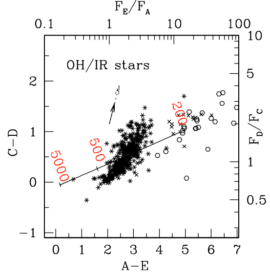
Fig. 17. MSX colour-colour plot as in Fig. 5 of Lumsden et al. (2002) for the OH/IR sample of Sevenster (2002). Symbols are as in Fig. 16, plus crosses which represent late post-AGB stars, following the classification of Sevenster (2002).
