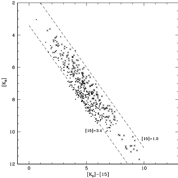
Fig. 10. 2MASS K_S versus (K_S - [15]) or (K_S - D) . Filled circles indicate objects from the ISO GAL sample, for which we plot (K_S - [15]) ; and crosses indicate objects from the MSX sample, for which we plot (K_S - D) . The two dashed lines correspond to [15] = 3.4 and 1.0 mag.
