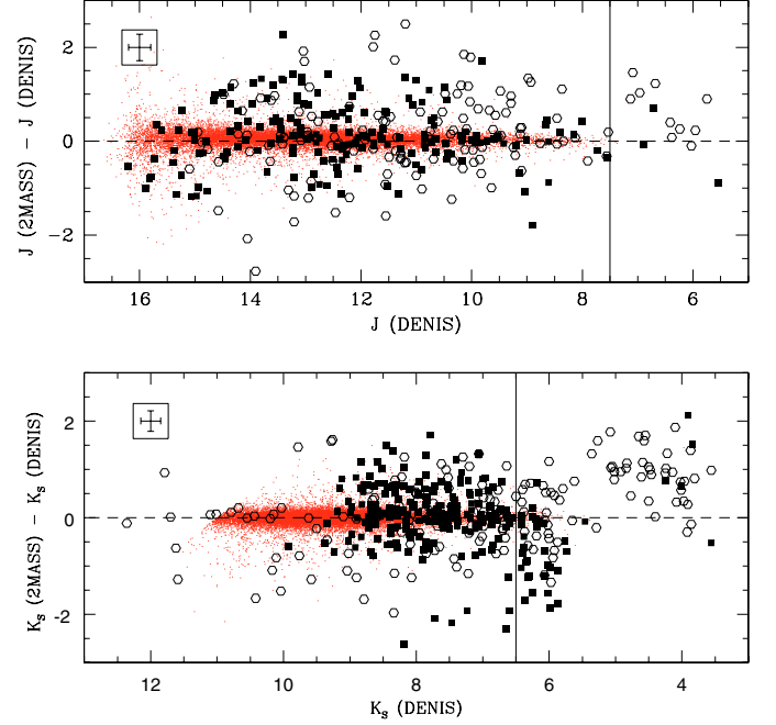
Fig. 11. Upper panel: difference between 2MASS and DENIS J magnitudes versus the DENIS J magnitude. Filled squares represent the ISOGAL SiO targets. For comparison small dots show ID-PSC and 2MASS associations obtained in several ISOGAL fields, which have a distribution of their J variations consistent with a Gaussian distribution centred at zero. No correction for offset in the photometric zeropoint was applied. Open circles represent the MSX targets, which have indications of variability at mid-infrared wavelengths. The error bars shown within the box are \pm 1\sigma mag. The vertical line indicates the DENIS saturation limit. Lower panel: comparison of the 2MASS and DENIS K_s magnitudes versus the DENIS K_s magnitude. Symbols are as in the top panel.
