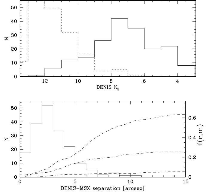
Fig. 4. Associations of our SiO MSX targets in the DENIS catalogue. Top panel: distribution of K_S magnitudes for the associations (continuum line) and for the chance associations (dashed line). Lower panel: the continuous line shows the distribution of angular separations. The dashed lines show the normalised cumulative distributions, f(r, m) , of chance associations found by misaligning the catalogue and MSX SiO targets, where we plot separately, starting from the bottom, the distributions of sources with K_S < 9 , 9 < K_S < 11 , and K_S > 11\ \text{mag} , respectively.
