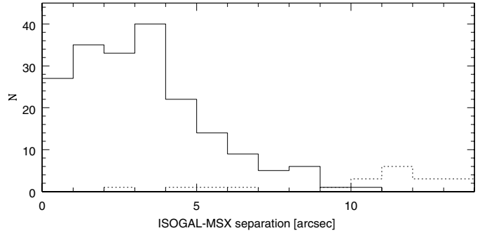
Fig. 2. Associations between our SiO ISOGAL targets and the MSX catalogues. The distribution of the angular separations (") between the ISOGAL and the MSX positions (continuum line). For comparison, the dashed line is the total distribution of the chance associations, found by performing five shifting experiments.
