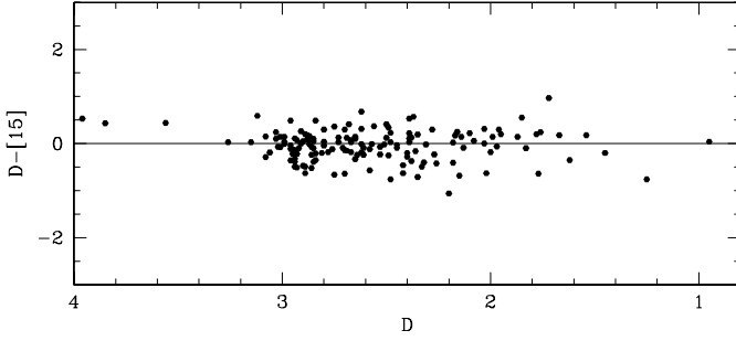
Fig. 3. Difference between the MSX band D magnitude, D , and the ISOCAM 15\ \mu\text{m} magnitudes, [15] , versus the D . Magnitude zero point in D band was taken from Egan et al. (1999). The continuous line is D - [15] = 0.0\ \text{mag} .
