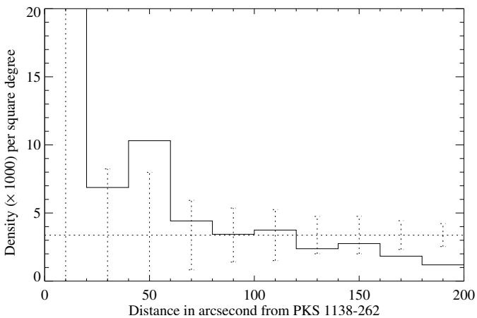
Fig. 11. Candidate \text{Ly}\alpha emitter ( EW_0 > 15 \text{ \AA} , \Sigma > 3 ) counts as a function of distance from the radio galaxy. The candidates are counted in circular bins of 20'' width. The error-bars represent Poissonian errors. The mean density ( 3.4 \times 1000 ) per square degree is indicated by the horizontal line.
