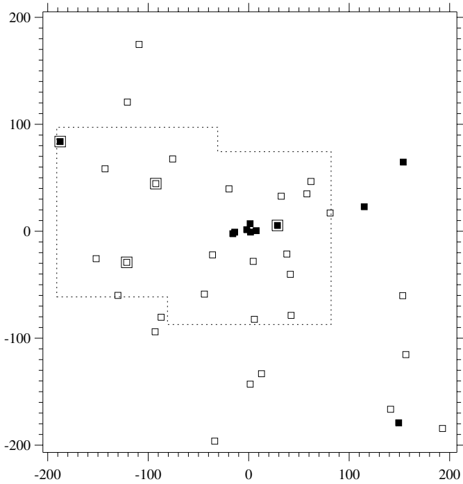
Fig. 10. Position plot for the 40 (11) \text{Ly}\alpha candidates with EW_0 > 15 \text{ \AA} and \Sigma > 3 (5) indicated by open (filled) squares. Large squares indicate candidates for which \text{H}\alpha emission has been detected (see Sect. 5.1). Axes are in arcseconds, the radio galaxy is at the origin. The dotted boxes indicate the borders of the two reduced ISAAC fields.
