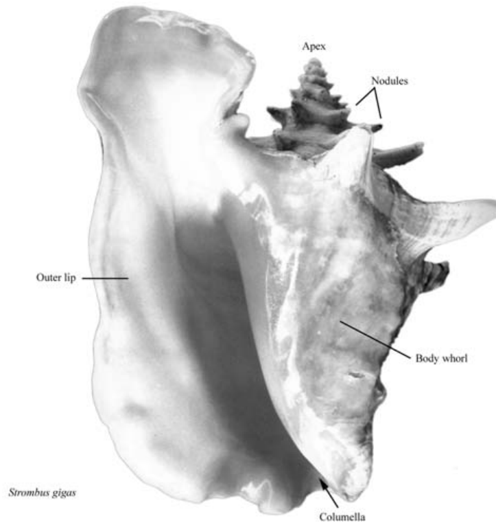
Fig. 2.1 Gastropod terms
