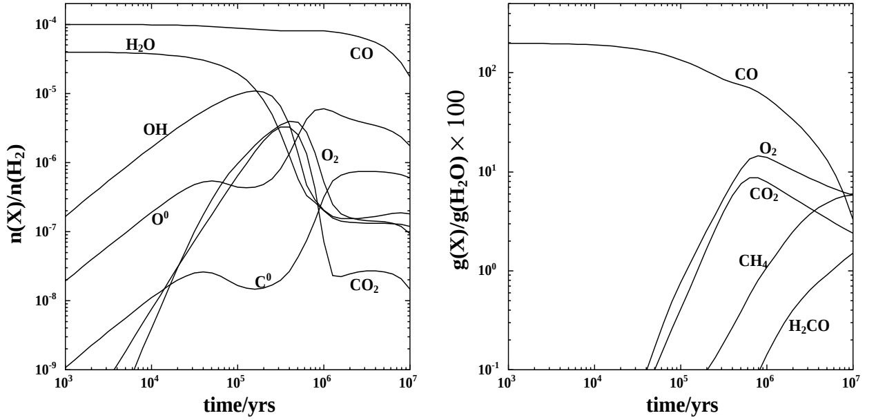
Fig. 2. As Fig. 1, but oxygen atoms accrete and are hydrogenated to water on grains: a) gas phase abundances, b) solid mantle fractions.
