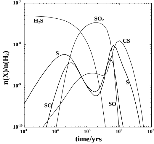
Fig. 5. Gas phase chemical evolution of the principal S-bearing species in the model of Fig. 3.
