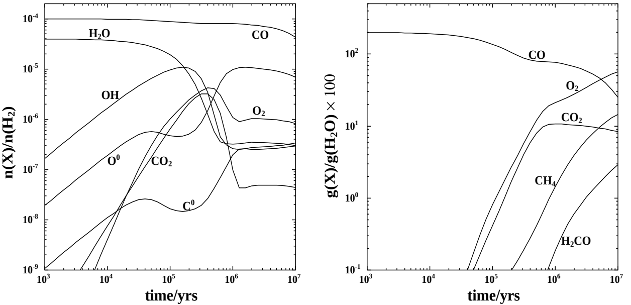
Fig. 1. Gas-grain chemical evolution of the principal atoms and molecules in the reference model: a) gas phase abundances, b) solid mantle fractions.
