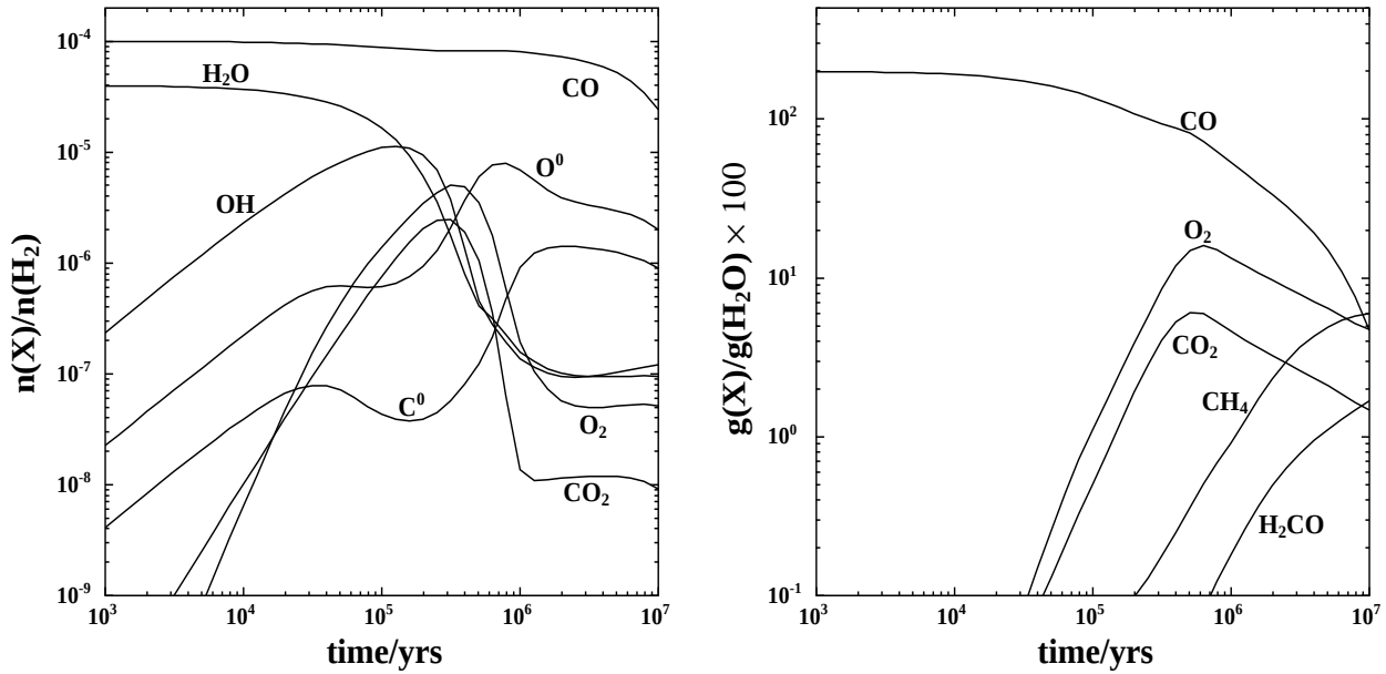
Fig. 3. As Fig. 2, but photochemistry due to the Prasad-Tarafdar radiation field was included: a) gas phase abundances, b) solid mantle fractions.
