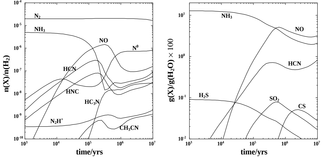
Fig. 4. Gas-grain chemical evolution of the principal N-bearing species in the model of Fig. 3: a) gas phase abundances, b) solid mantle fractions, including those of S-bearing molecules.
