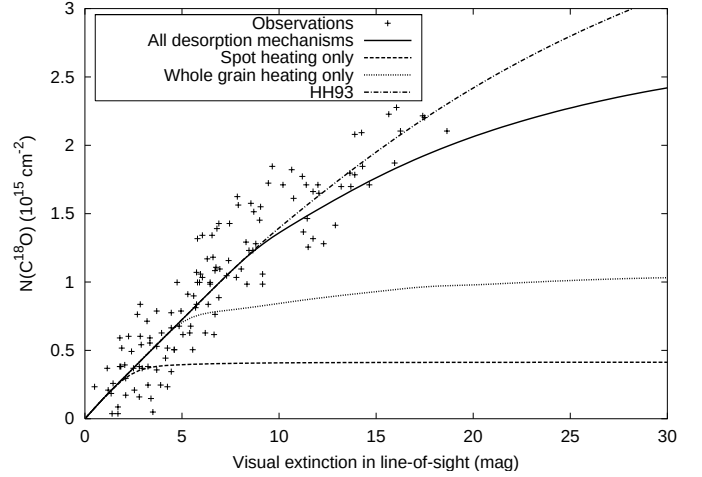
Fig. 9. The column density of \text{C}^{18}\text{O} as a function of visual extinction A_V using the desorption due to cosmic-ray whole grain heating only (dotted line), cosmic-ray spot heating only (dashed line) and chemical energy released from free radicals combined with the other two (solid line). The points are the observations of L977 made by Alves et al. (1999). The dash-dotted line is the calculation using the desorption due to cosmic-ray heating by the Hasegawa & Herbst (1993) approximation (see text for details).
