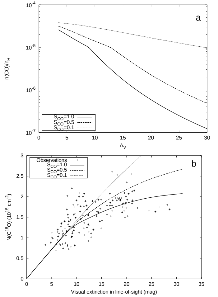
Fig. 14. The relative abundance of gaseous CO to total hydrogen a) and the C^{18}O column density b) as a function of visual extinction A_V for different values of the sticking coefficients S_{CO} of CO.
