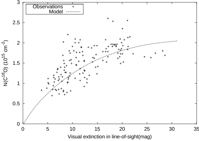
Fig. 10. The total \text{C}^{18}\text{O} column density along the line of sight as a function of visual extinction for the dense core of IC 5146. The points are the observations of IC 5146 made by Kramer et al. (1999).
