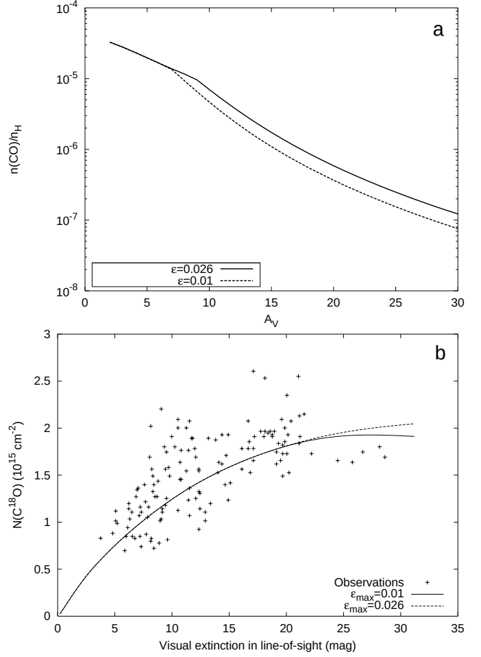
Fig. 12. The relative abundance of gaseous CO to total hydrogen a) and the \text{C}^{18}\text{O} column density b) as a function of visual extinction along the line of sight for different maximum radical concentration \epsilon_{\text{max}} .
