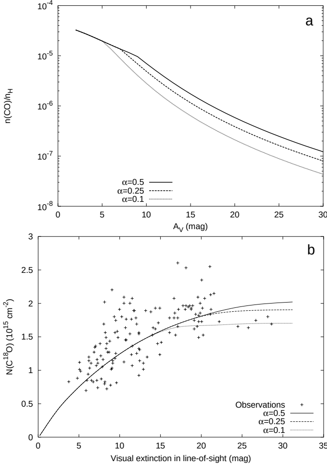
Fig. 13. The relative abundance of gaseous CO to total hydrogen a) and the C^{18}O column density b) as a function of visual extinction A_V for different values of the efficiency of free radical production by UV photons \alpha .
