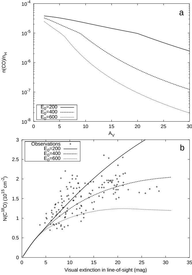
Fig. 11. The relative abundance of gaseous CO to total hydrogen a) and the \text{C}^{18}\text{O} column density b) as a function of visual extinction along the line-of-sight for different cosmic-ray energy spectra.
