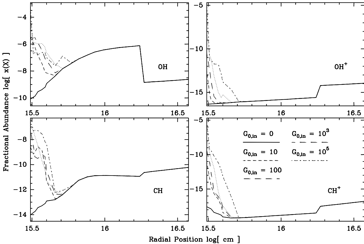
Fig. 5. Depth-dependent fractional abundances of the hydrides OH, OH + , CH and CH + for different UV fluxes.
