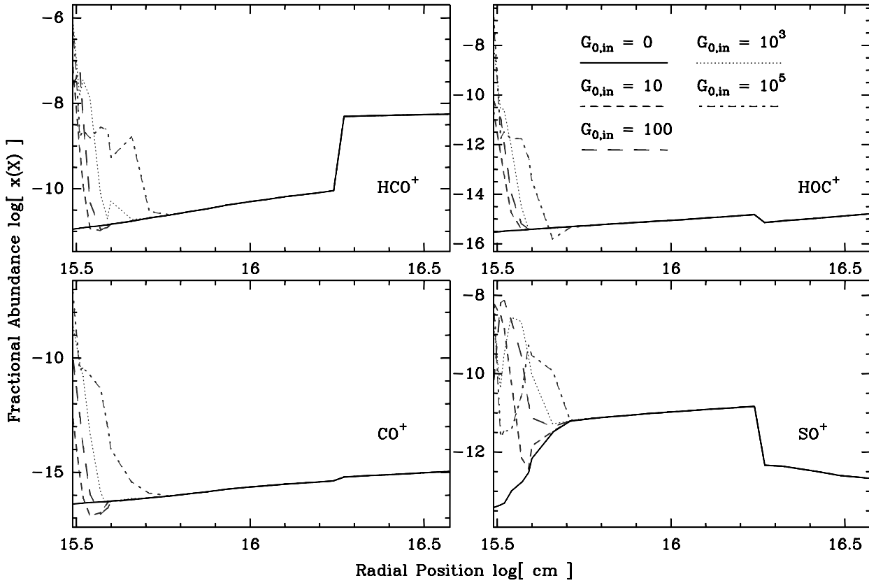
Fig. 4. Depth-dependent fractional abundances of HCO + , HOC + , CO + and SO + for different UV fluxes.
