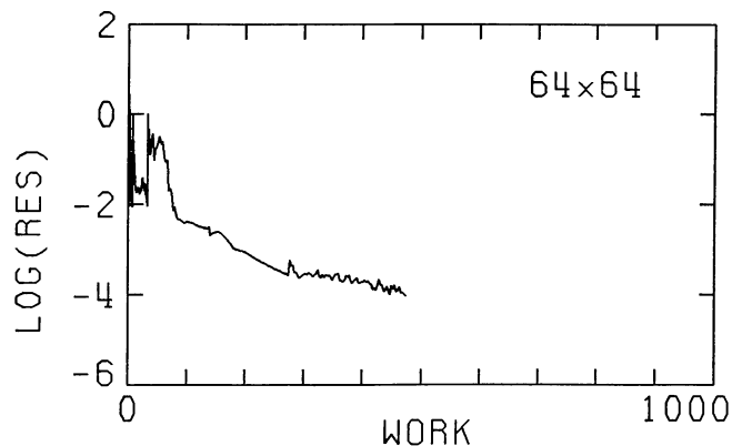
Fig. 7. The convergence history of a 64 \times 64 second-order Type II solution, with varying central \rho_c .
