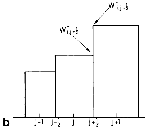
Fig. 1.b One-dimensional cross-cut at constant \phi_i for a first-order scheme, showing one component of the vector of state quantities. The boundary values w_{i,j+1/2}^+ , etc., are obtained by zeroth-order interpolation from the cell averages w_{ij} . c As b , but for a second-order-accurate scheme. The boundary values are obtained by first-order interpolation. The discrete state-quantities are assumed to be piecewise linear
