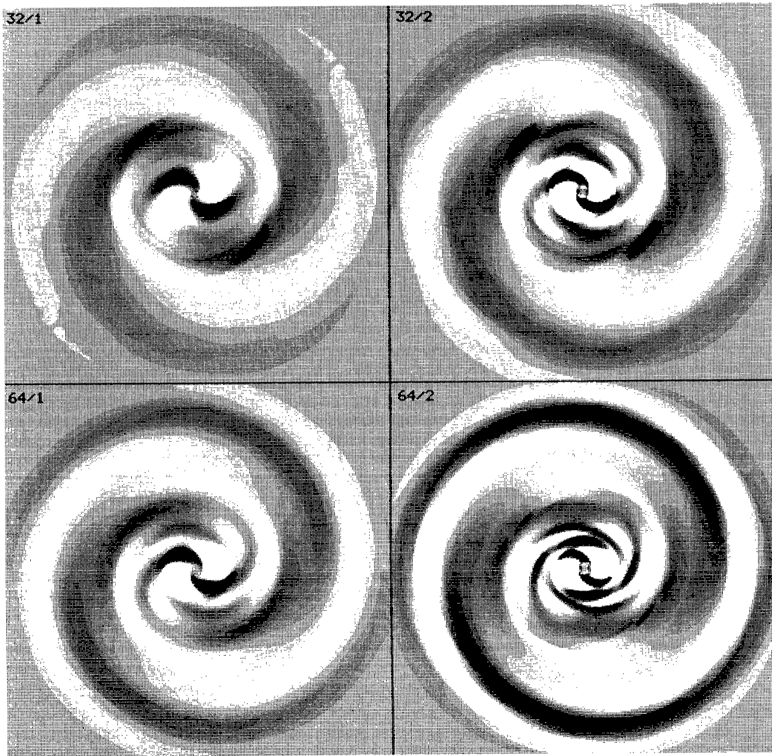
Fig. 4. The logarithm of the density scaled by the average density per ring, \ln(\varrho/\langle\varrho\rangle) . A darker shade corresponds to a higher density. The upper row shows the solutions on a 32 \times 32 grid, the lower on a 64 \times 64 grid. The results on the left are first-order- and on the right second-order-accurate. Each side of a figure corresponds to 40 units of length. The ILR is at 1.22, CR at 8.36 and the OLR at 15.49
