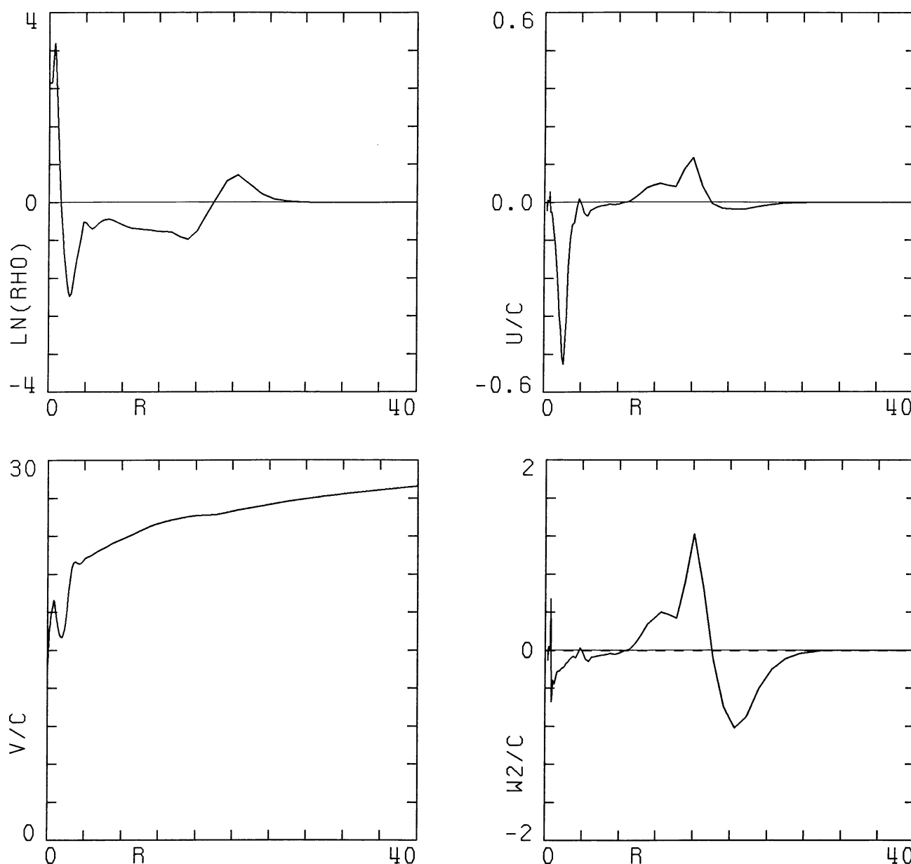
Fig. 8. Averages per ring for the 64 \times 64 second-order Type II solution. The average central density finally becomes \rho_c = 12.4
