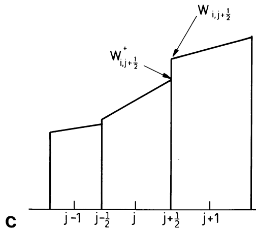
Fig. 1.b One-dimensional cross-cut at constant \phi_i for a first-order scheme, showing one component of the vector of state quantities. The boundary values w_{i,j+1/2}^+ , etc., are obtained by zeroth-order interpolation from the cell averages w_{ij} . c As b , but for a second-order-accurate scheme. The boundary values are obtained by first-order interpolation. The discrete state-quantities are assumed to be piecewise linear
