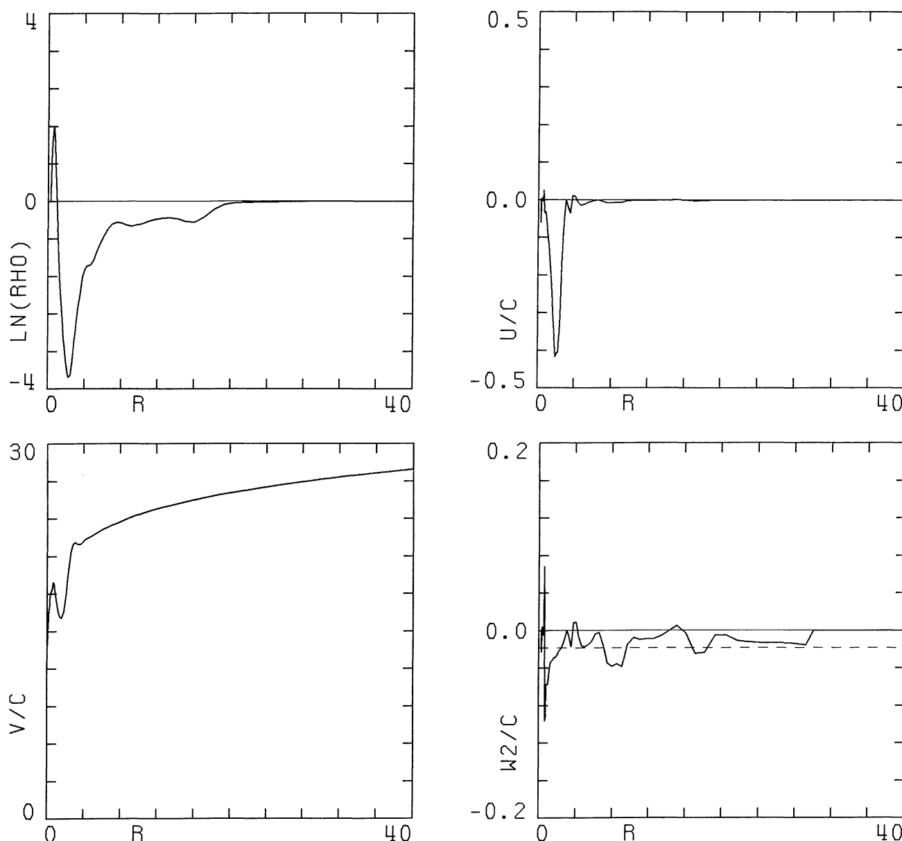
Fig. 5. Averages per ring for the 64 \times 64 second-order Type I solution with a fixed average central density \varrho_c = 1 . The dashed line in the plot of w_2/c indicates the average value of the a_{j+1/2} , that are constant within 1% for all j . The deviations from this line give an impression of the numerical discretization error
