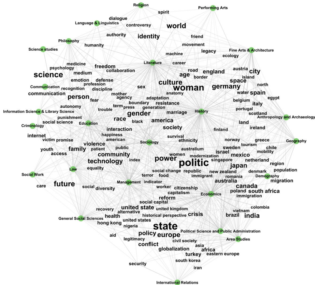
Figure 2. Bimodal network of SSH specialties and noun phrases that are weekly associated (1980-2015).
