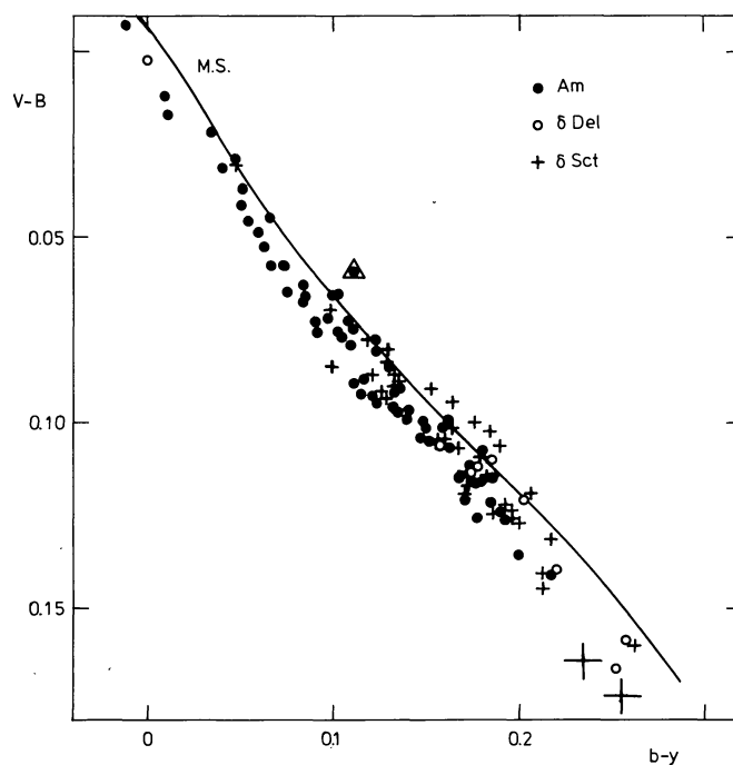
Fig. 4. The b-y/V-B diagram for Am, \delta Del, and \delta Sct stars. The full curve is the relation for normal main sequence stars of type A/F
