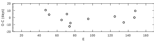
Fig. 10. O-C diagram for all T_{\max} data listed in Table 4.
