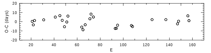
Fig. 9. O–C diagram for all T_{\text{min}} data listed in Table 3.
