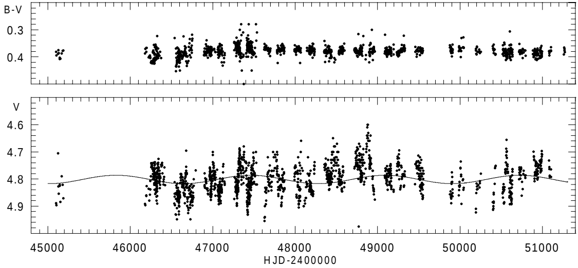
Fig. 5. Combined V light curve. The continuous line represents the best-fitting sine curve with P = 1630 days and amplitude 0^{\text{m}}015 (fit on the basis of all data collected after JD 2446000).
