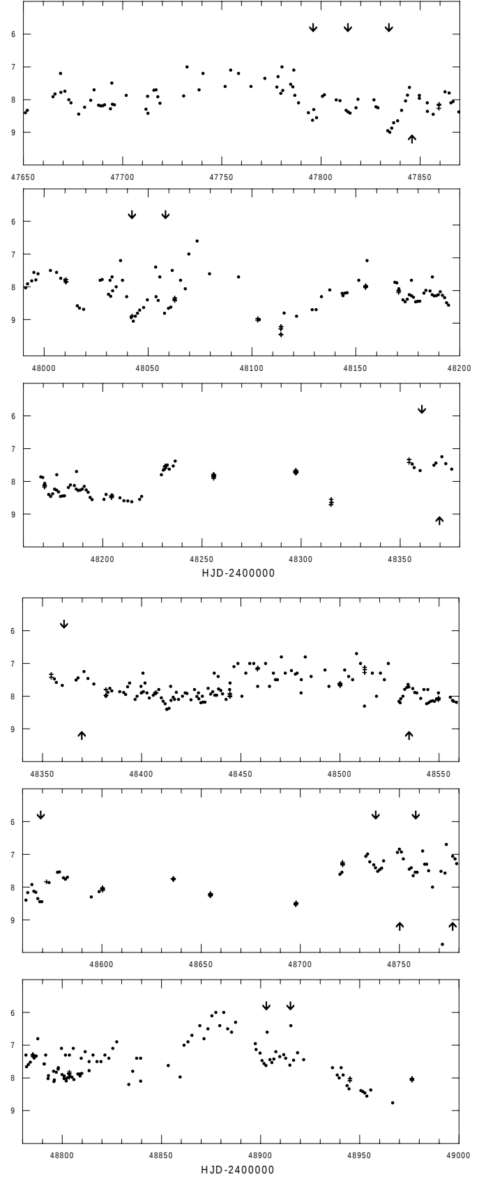
Fig. 7. V light curve of P Cyg.
