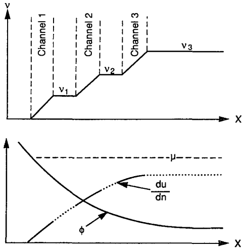
FIG. 1. Schematic drawing of the variation in filling factor v , electrostatic potential \phi , and chemical potential du/dn , at a smooth boundary in a 2DEG. The dashed line in the bottom panel denotes the constant electrochemical potential \mu = \phi + du/dn . The dotted intervals indicate a discontinuity (energy gap) in du/dn , and correspond in the top panel to regions of constant fractional filling factor v_p which spatially separate the edge channels.
