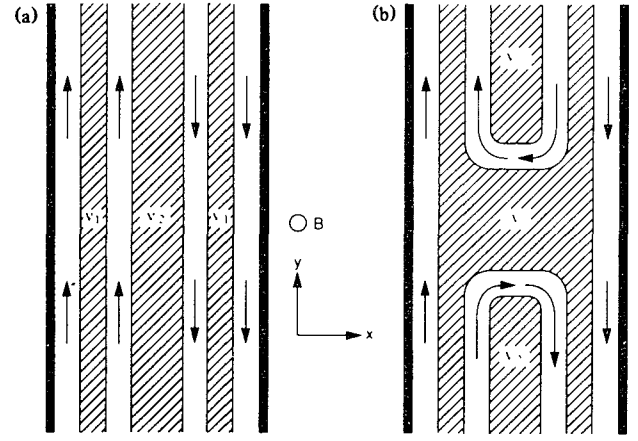
FIG. 2. Schematic drawing of the incompressible bands (hatched) of fractional filling factor v_p , alternating with the edge channels (arrows indicate the direction of electron motion in each channel). (a) A uniform conductor; (b) a conductor containing a barrier of reduced filling factor (as in the experiment of Ref. 10).
