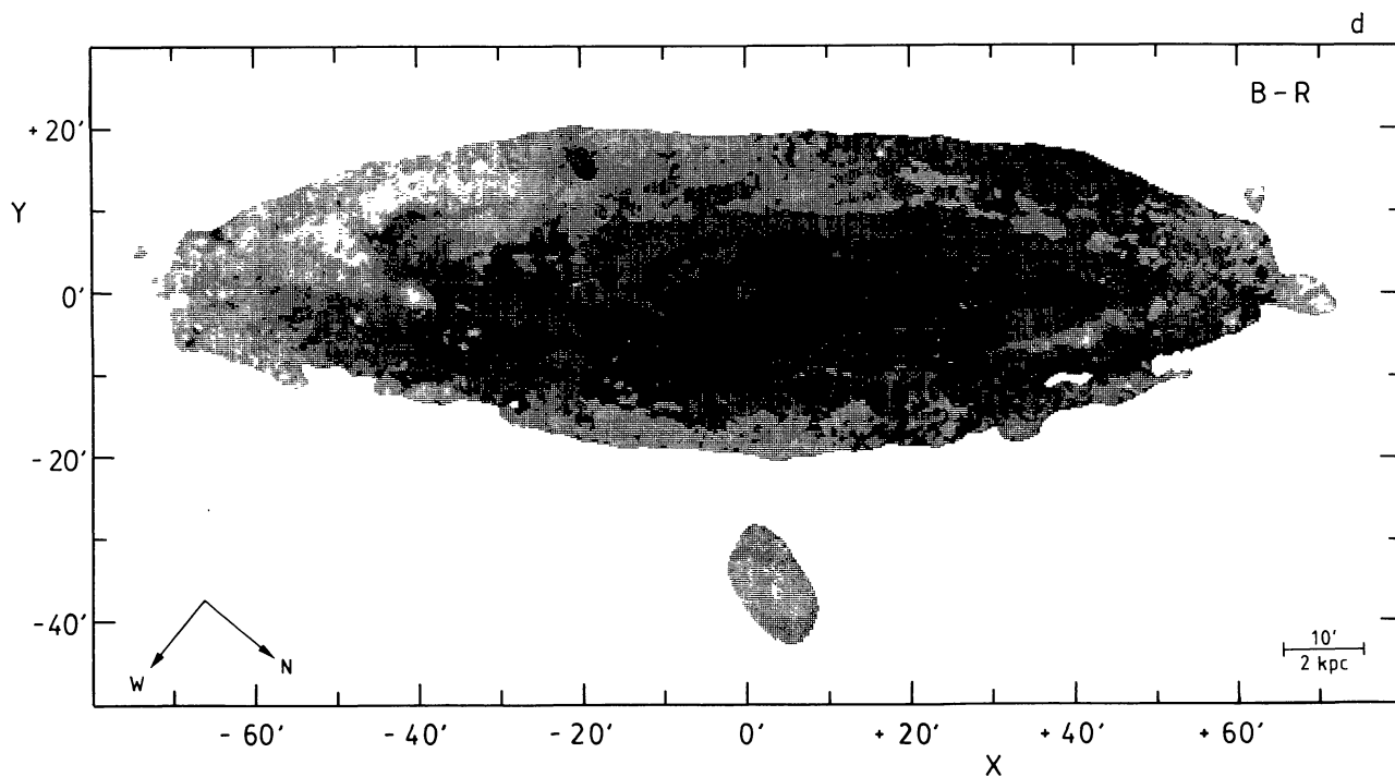
FIGURE 11. — (d) B-R , gray levels (from light to dark): < 1.24 , 1.24-1.36 , 1.36-1.48 , 1.48-1.60 , 1.60-1.72 , 1.72-1.84 , 1.84-1.96 , > 1.96 .
