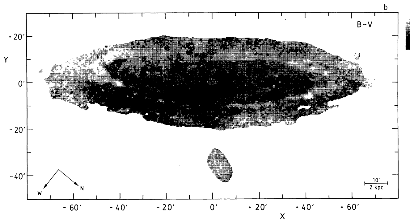
FIGURE 11. — (b) B-V , gray levels (from light to dark): < 0.66 , 0.66-0.74 , 0.74-0.82 , 0.82-0.90 , 0.90-0.98 , 0.98-1.06 , 1.06-1.14 , > 1.14 .
