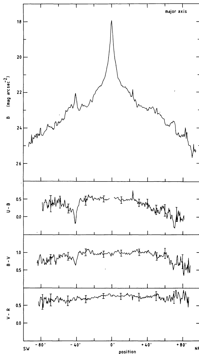
FIGURE 10. — (a) Major axis. The bright blue peak near -40' is the OB association NGC 206. On the opposite side spiral-arm crossings can also be seen. The sharp peak near +22' is a foreground star that was apparently missed by the automatic star removal procedure on the B map.
