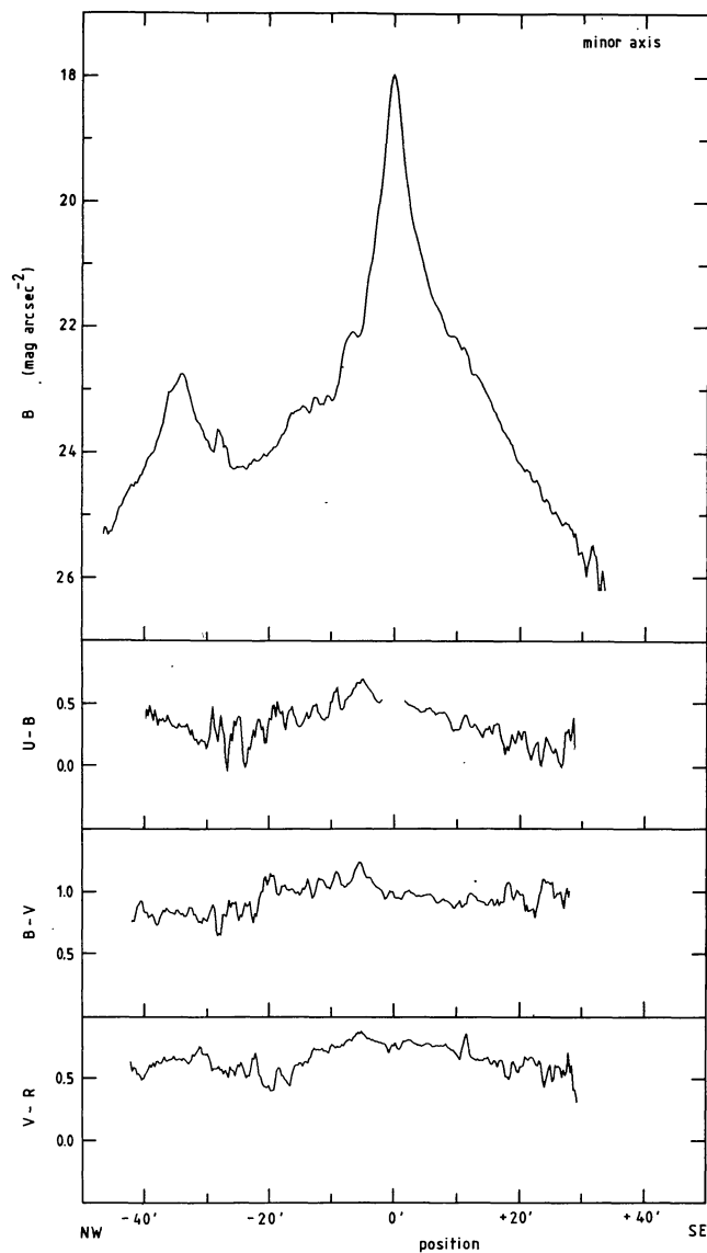
FIGURE 10. — (b) Minor axis. Dust lanes on the West side can be recognized as a reddening of the colors around -6' and -10' . The hump to the left is due to the elliptical companion NGC 205.
