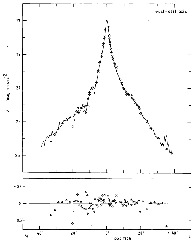
FIGURE 9. — Comparison of our V photometry (60" aperture) with published data for the West-East axis of M31. See figure 6 for details. References: triangles - de Vaucouleurs (1958); diamonds - Burgess (1976); crosses - Sharov and Lyutyj (1980).
