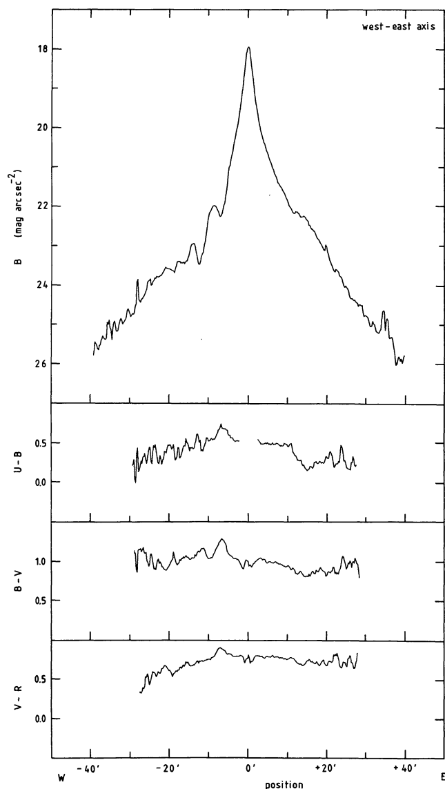
FIGURE 10. — (c) West-East axis. Red features on the West side correspond to strong dust lanes. The crossing of the bright NE arm around 10 kpc from the nucleus is apparent in the U-B and B-V profiles near +10' to +20' .
