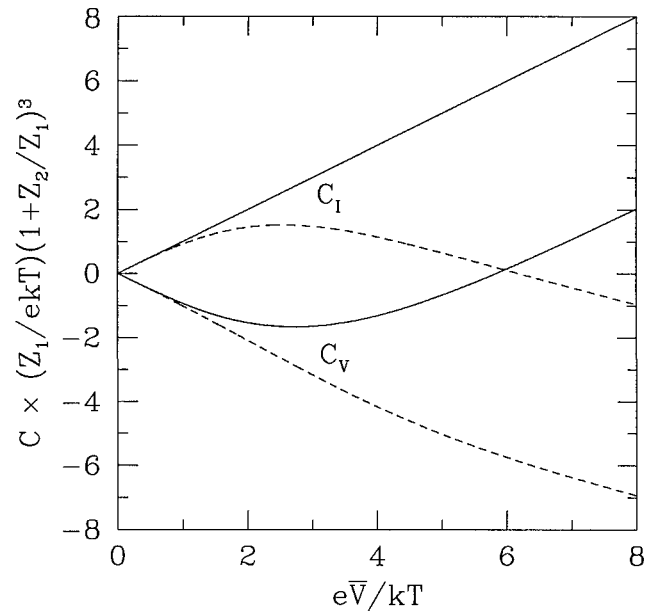
FIG 2 Voltage dependence of the third cumulants C_I and C_V of current and voltage for a tunnel junction (resistance Z_1 ) in series with a macroscopic resistor Z_2 . The two solid curves are for Z_2/Z_1 \rightarrow 0 and the dashed curves for Z_2/Z_1 = 1 . The curves are computed from Eq (13) for T_1 = T_2 \equiv T . The high voltage slopes are the same for C_I and C_V , while the low voltage slopes have the opposite sign.
