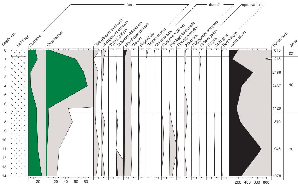
Figure 18.4 Pollen diagram Schipluiden 16 North. Percentages (black) and percentages 10x (grey). Dominant local pollen taxa indicated in colour.
