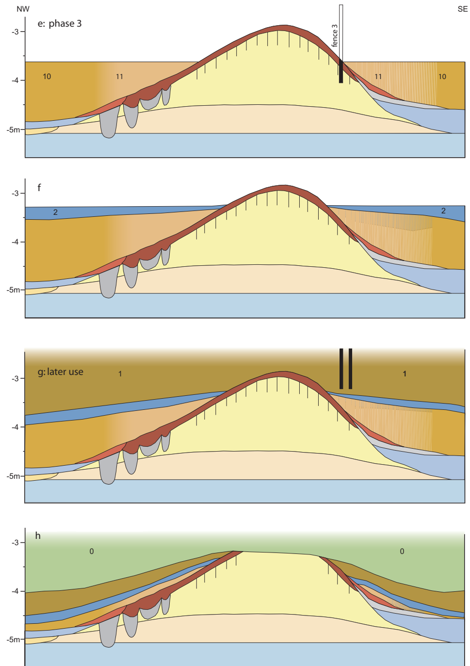
Figure 2.7 Schipluiden-Harnaschpolder, schematic representation of landscape development before, during and after the period of occupation. Only the newly formed units have been numbered. Soil formation indicated by shading.
