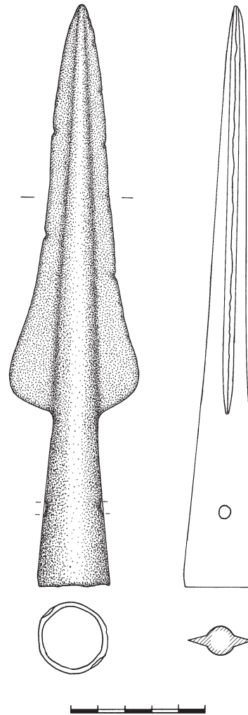
Figure 7.12 Flame-shaped spearhead from the river Meuse near Wesseem (scale 1:2; coll. Niessen).
