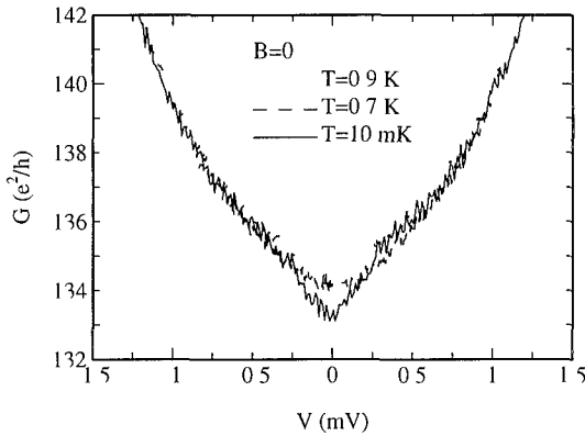
Fig. 5 Differential conductance as a function of applied voltage at three different temperatures. Experimental data by Lennsen et al. for a two dimensional electron gas with superconducting contacts. The dip around zero voltage, which is superimposed on the broad minimum at the lowest temperature, is attributed to the enhancement of weak localization by Andreev reflection. (From ref. [40].)
