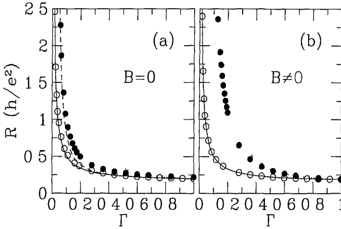
Fig 8 Filled circles Numerically calculated resistance R_{NS} of a disordered NS junction versus the transmission probability per mode \Gamma of the tunnel barrier at the NS interface. Open circles Resistance R_N of the same junction in the normal state. (a) is for zero magnetic field, (b) is for a flux of 10 h/e through the disordered region. The dotted and solid curves are the classical eqs (5.1) and (5.2). The dashed curve is the theory of ref [52] which for \Gamma \gg l/L \approx 0.12 coincides with eq (5.3). (From ref [39])
