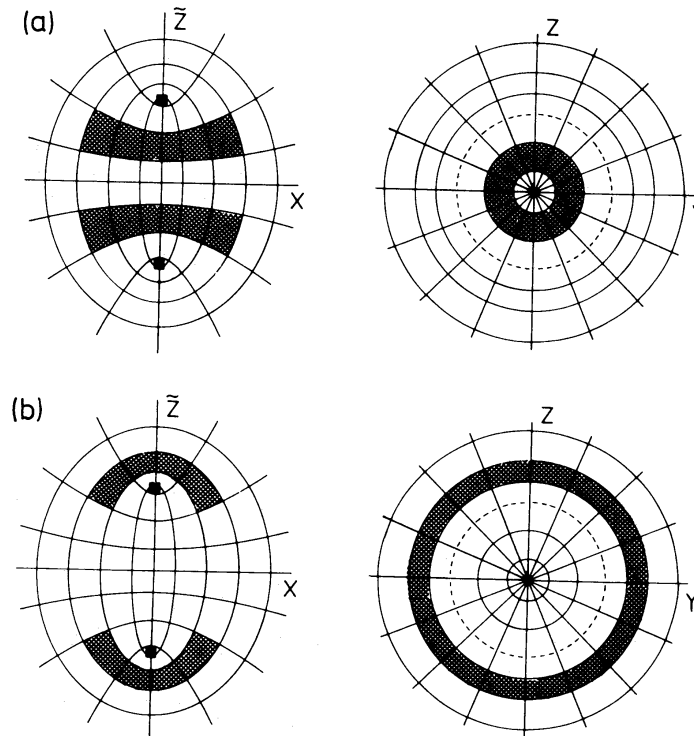
Figure 20. Cross-section with a meridional plane and with the equatorial plane of the volumes allowed to the two general orbits by the values of the integrals of motion. The focal circle is dashed. The filled squares are the foci. (a) Inner long axis tube; (b) outer long axis tube.
