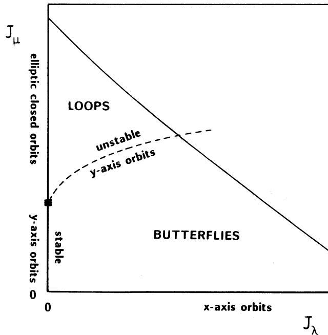
Figure 30. Action-diagram for the orbits in the (x, y) -plane of the perfect ellipsoid. The locations of the various orbit families are indicated. The filled square represents the y -axis orbit that just reaches the foci of the elliptic coordinates. The figure is equivalent to Fig. 10. The drawn curve is a line of constant energy.
