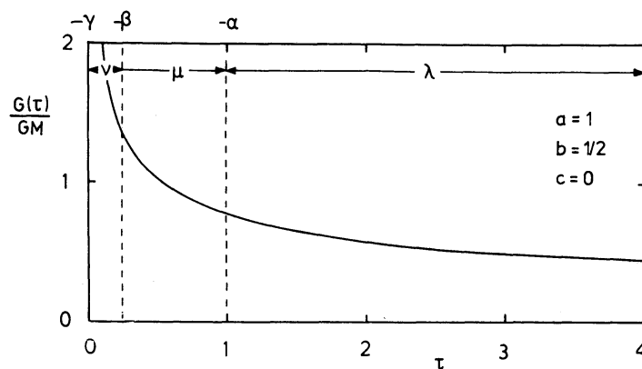
Figure 5. The function G(\tau) for a=1, b=1/2 and c=0 .
