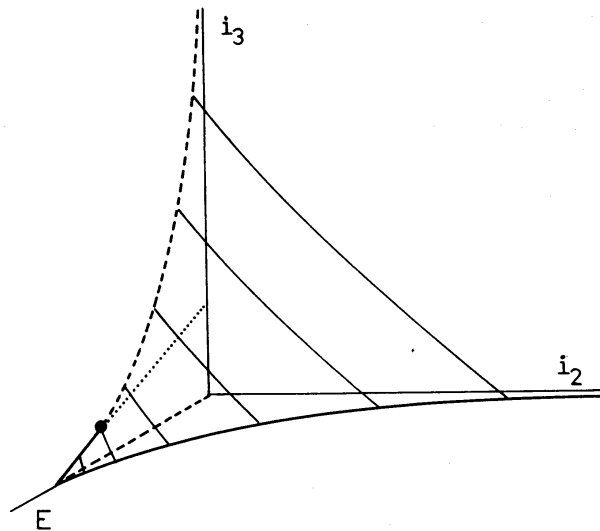
Figure 25. Three-dimensional classification of orbits in the perfect oblate spheroid in terms of the integrals E , i_2 = \frac{1}{2}l_z^2 and i_3 . Each point within the volume shown corresponds to a bound orbit. Dashed and dotted lines have the same meaning as in Fig. 13.
