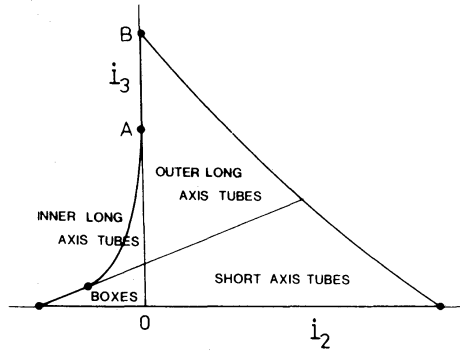
Figure 18. Cross-section of Fig. 17 with a plane of constant E ( E_4 < E < 0 ).
