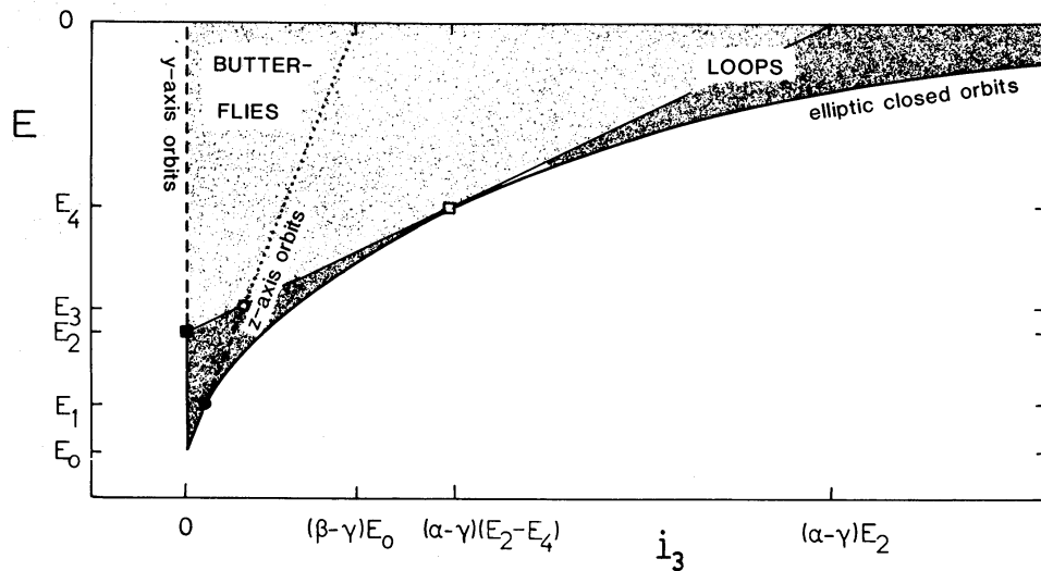
Figure 16. Classification of orbits in the (y, z) -plane of the perfect ellipsoid in terms of the integrals E and i_3 . Shadings, dashed and dotted lines have the same meaning as in Fig. 13.
