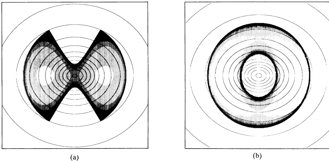
Figure 27. Densities of two orbits in the (x, y) -plane. The curves are contours of constant potential energy. A darker shading indicates a higher density. (a) Butterfly; (b) loop.
