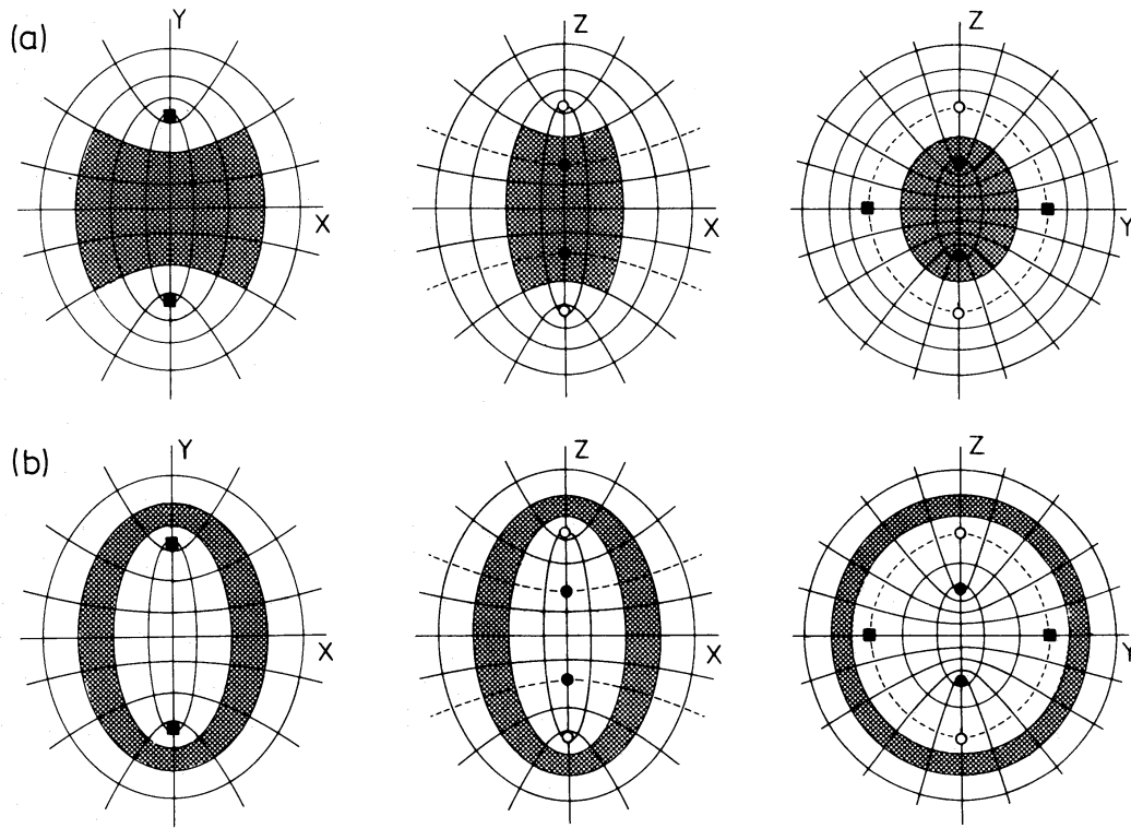
Figure 12. Cross-sections with the principal planes of the volume allowed by the values of the integrals of motion for the two unstable orbits in the (x, z) -plane of the perfect ellipsoid. (a) Unstable butterfly; (b) unstable loop.
