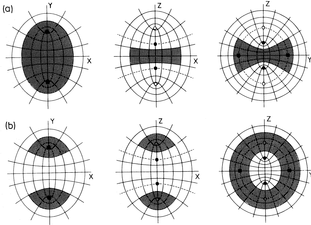
Figure 15. Cross-sections with the principal planes of the volume allowed by the values of the integrals of motion for the two unstable orbits in the (y, z) -plane of the perfect ellipsoid. (a) Unstable butterfly; (b) unstable loop.
