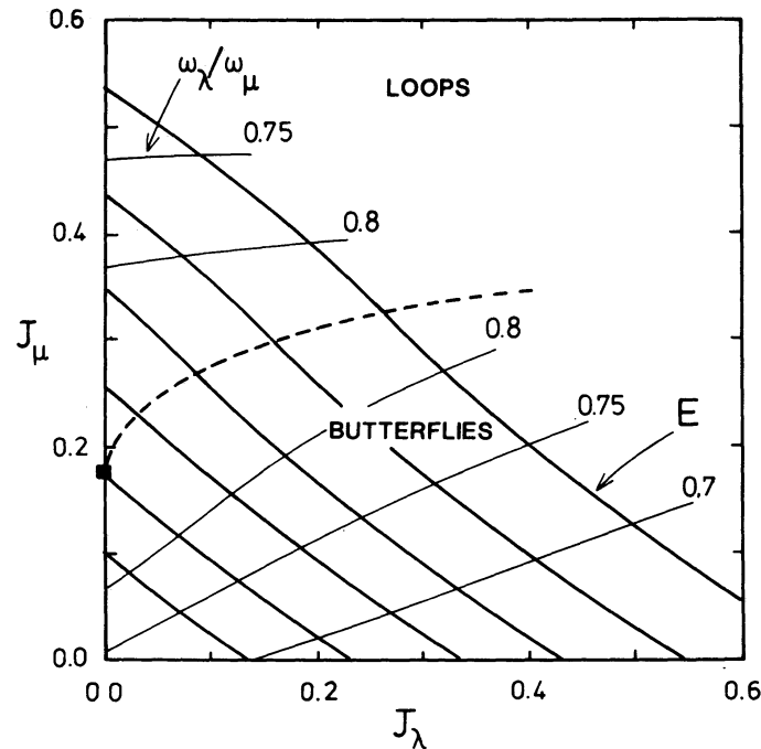
Figure 32. Action-diagram with curves of constant frequency \omega_\lambda/\omega_\mu (thin), and curves of constant energy (thick). Energy increases towards the upper right.
