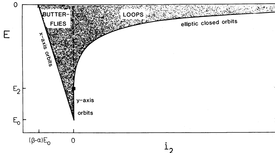
Figure 10. Classification of orbits in the (x, y) -plane of the perfect ellipsoid in terms of the integrals E and i_2 . Each point in the shaded region corresponds with a bound orbit. The dashed line represents the unstable y -axis orbit.
