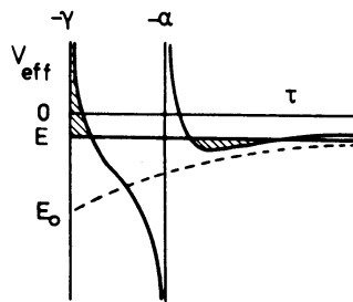
Figure 23. Effective potential curve for a short axis tube in the perfect oblate spheroid. The dashed curve is -G(\tau) .
