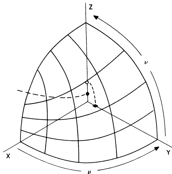
Figure A1. Behaviour of the ellipsoidal coordinates at large radii. The intersections of the hyperboloids of one ( \mu ) and two ( \nu ) sheets with a sphere of radius r \gg 1 are shown. The dashed curves indicate the focal ellipse and the focal hyperbola.
