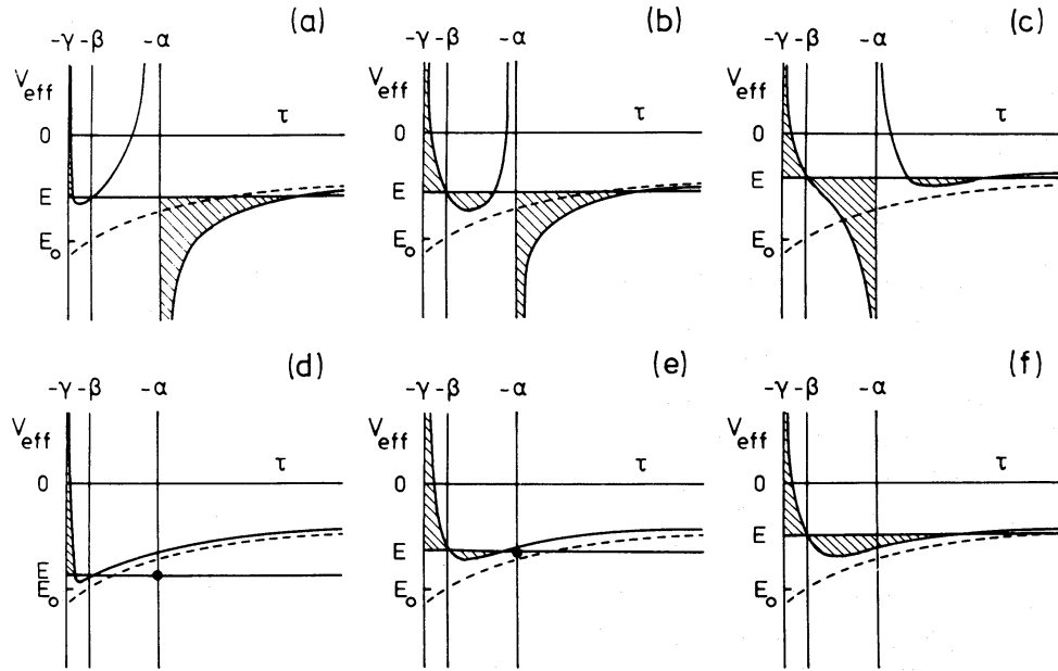
Figure 11. Effective potential curves for orbits in the (x, z) -plane of the perfect ellipsoid. (a) Stable butterfly; (b) unstable butterfly; (c) unstable loop; (d) stable z -axis orbit; (e) unstable z -axis orbit; (f) twice unstable z -axis orbit.
