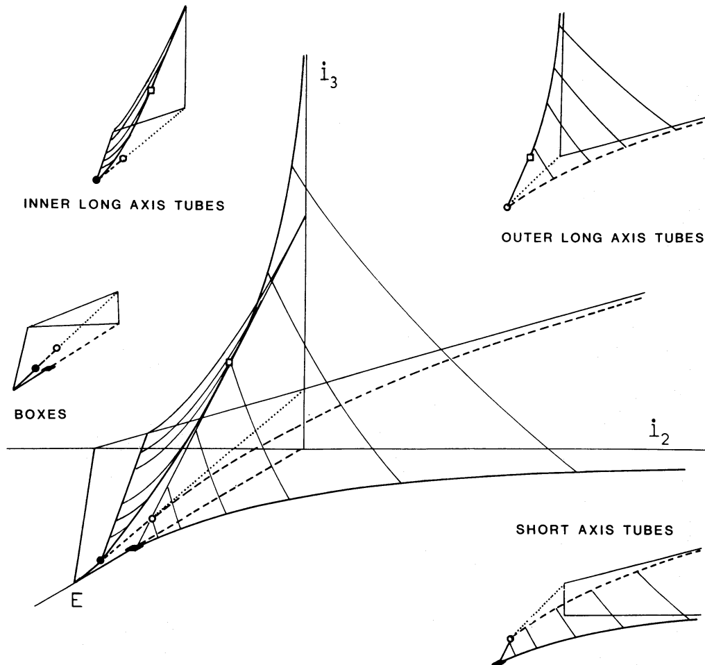
Figure 17. Three-dimensional classification of orbits in the perfect ellipsoid in terms of the integrals E , i_2 and i_3 . Each point within the volume shown corresponds with a bound orbit. Dashed and dotted lines have the same meaning as in Fig. 13. The three planar cross-sections in which each point corresponds to an orbit in one of the principal planes, are shown with more detailed explanations in Figs 10, 13 and 16. They separate the four volumes, identified by separate insets, that correspond with the four families of three-dimensional orbits.
