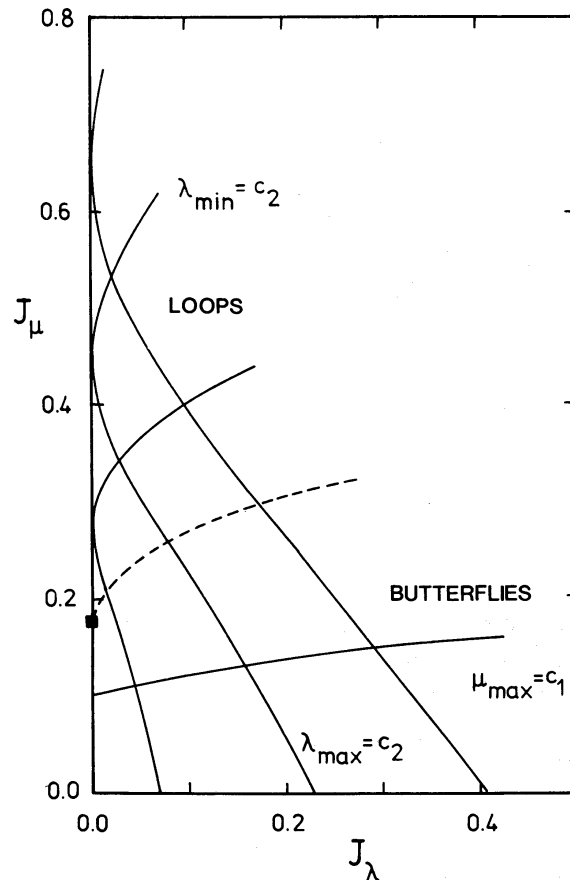
Figure 33. Action-diagram with curves of constant values of \lambda_{\max} , \lambda_{\min} and \mu_{\max} .
