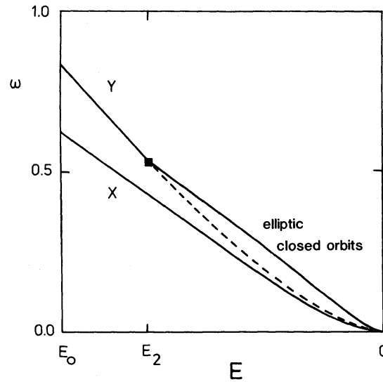
Figure 31. Frequencies of the simple periodic orbits in the (x, y) -plane of the perfect ellipsoid as function of the energy. The dashed line indicates the unstable y -axis oscillation.
