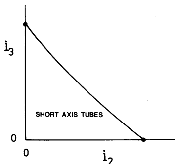
Figure 26. Cross-section of Fig. 25 with a plane of constant E .
