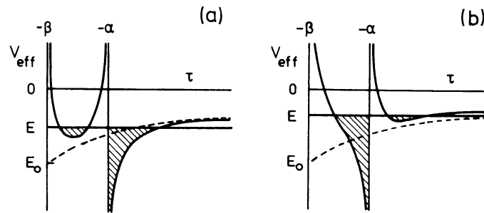
Figure 19. Effective potential curves for the two families of general orbits in the perfect prolate spheroid. The dashed curve is -G(\tau) . (a) Inner long axis tube; (b) outer long axis tube.
