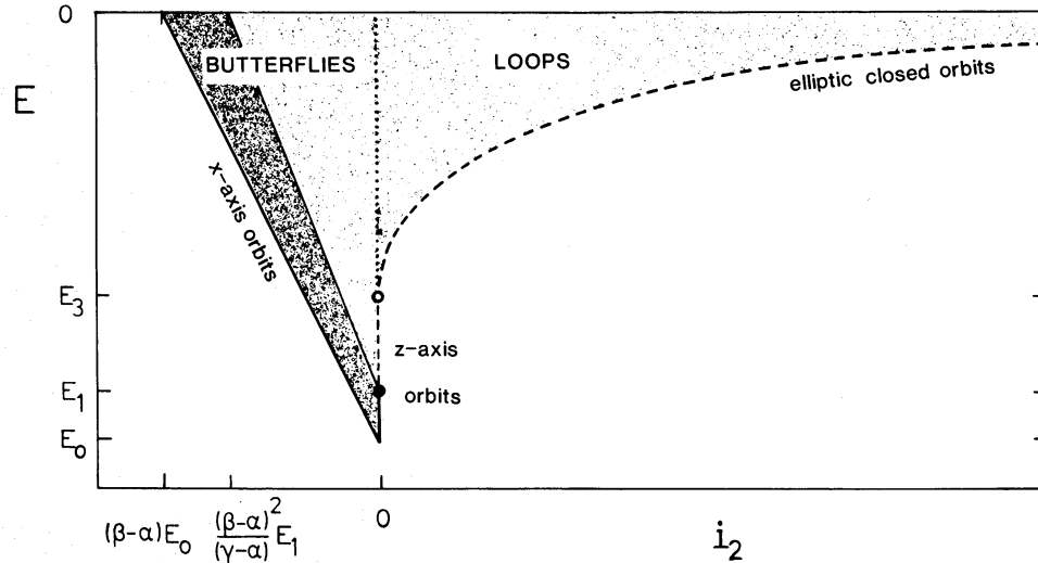
Figure 13. Classification of orbits in the (x, z) -plane of the perfect ellipsoid in terms of the integrals E and i_2 . The shaded area corresponds with stable bound orbits, the light shaded area with unstable bound orbits. Dashed lines represent once unstable periodic orbits, the dotted line twice unstable periodic orbits.
