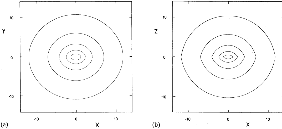
Figure 6. Equipotential curves in two principal planes for the perfect elliptic disc, for a=1 , b=1/2 and c=0 . (a) (x, y) -plane; (b) (x, z) -plane.
