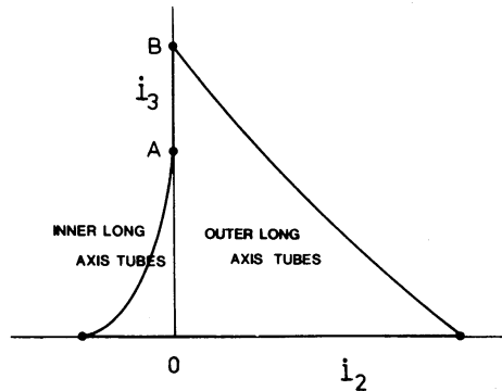
Figure 22. Cross-section of Fig. 21 with a plane of constant E ( E_4 < E < 0 ).
