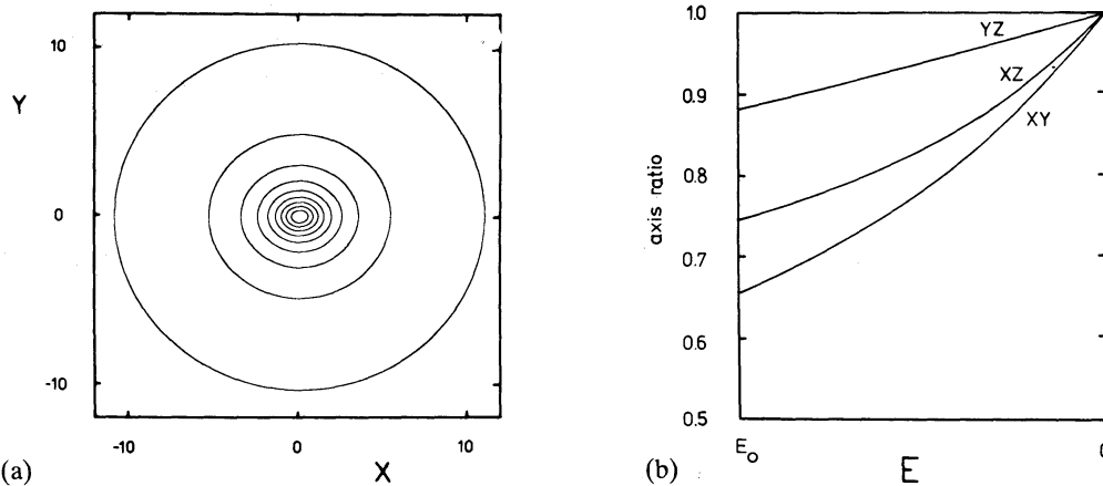
Figure 4. (a) Equipotential curves in the (x, y) -plane of the perfect ellipsoid. Contours are shown for E/V(0, 0, 0)=0.9, \dots, 0.1 , in intervals of 0.1. (b) Axis ratios of the equipotential curves in all three principal planes as function of the value of the potential energy.
