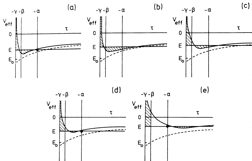
Figure 14. Effective potential curves for orbits in the (y, z) -plane of the perfect ellipsoid. (a) Stable butterfly; (b) unstable butterfly; (c) unstable loop; (d) inner stable loop; (e) outer stable loop.
