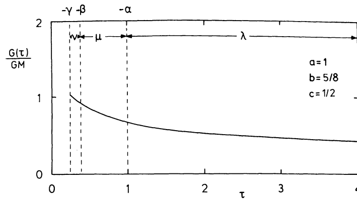
Figure 3. The function G(\tau) for a=1 , b=5/8 and c=1/2 .
