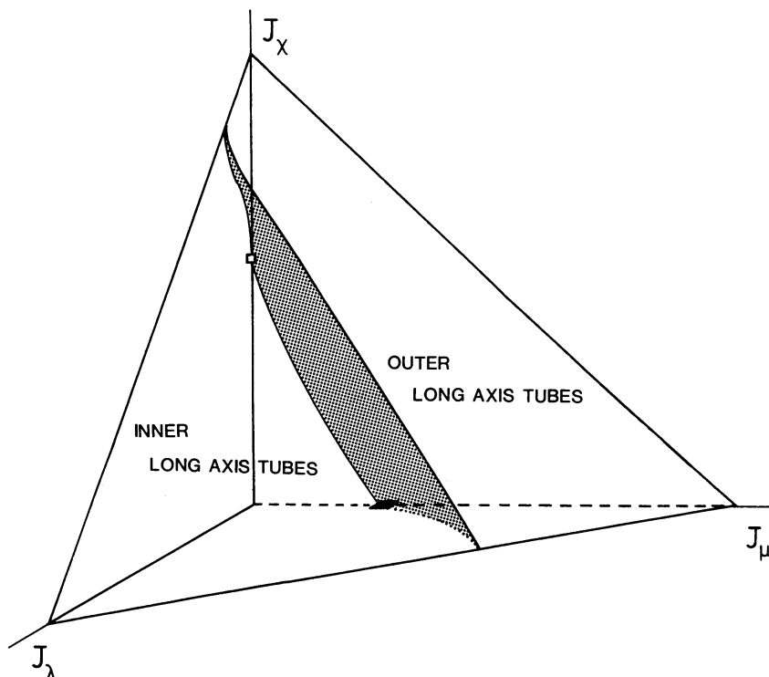
Figure 34. Action-diagram for the orbits in the perfect prolate spheroid. The diagram is equivalent to Fig. 21.
