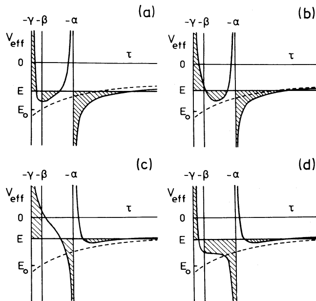
Figure 7. Effective potential curves for the four families of general orbits in the perfect ellipsoid. The dashed curve is -G(\tau) . The area between the line of constant E and V_{\text{eff}}(\tau) in the intervals where equation (54) is satisfied is hatched. (a) Box; (b) inner long axis tube; (c) outer long axis tube; (d) short axis tube.
