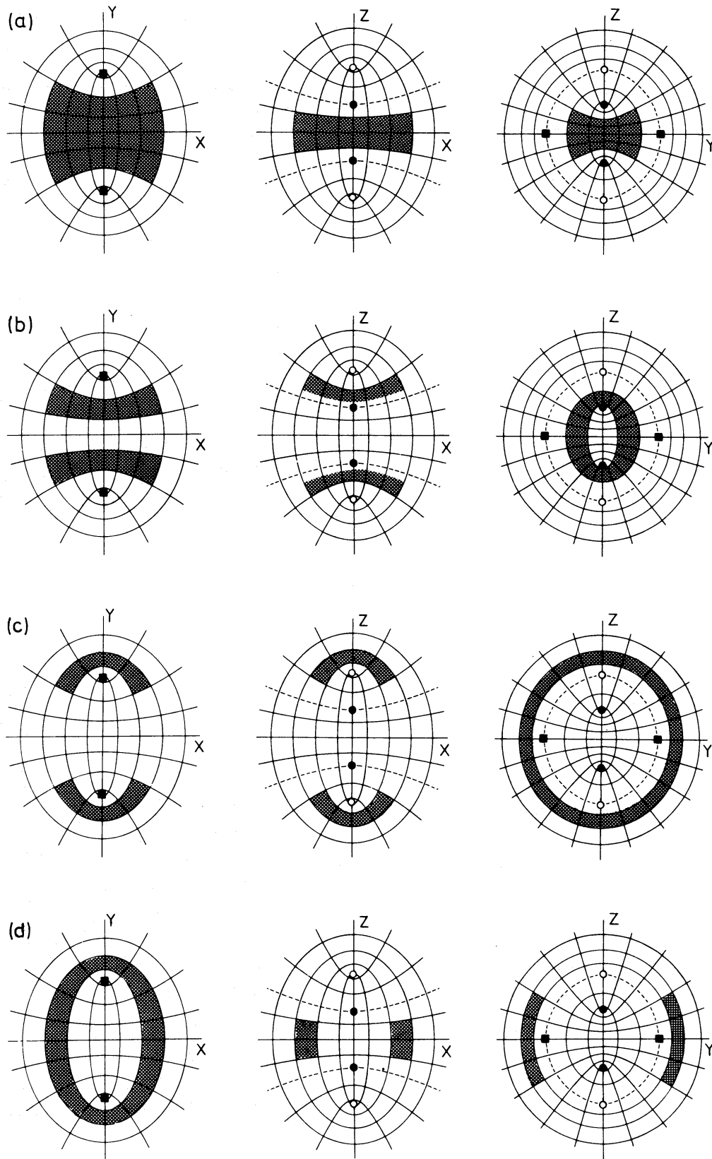
Figure 8. Cross-sections with the three principal planes of the volumes allowed to the four general orbits by the values of the integrals of motion. The dashed curves indicate the focal hyperbola [ (x, z) -plane] and the focal ellipse [ (y, z) -plane]. The foci are denoted by the same symbols as in Fig. 2. (a) Box orbit; (b) inner long axis tube; (c) outer long axis tube; (d) short axis tube.
