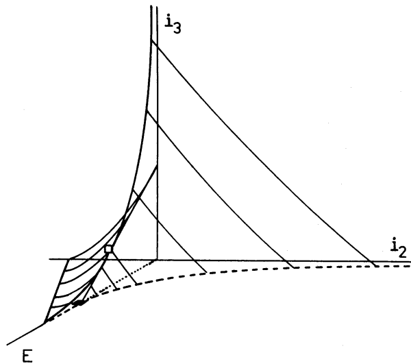
Figure 21. Three-dimensional classification of orbits in the perfect prolate spheroid in terms of the integrals E , i_2 and i_3 = \frac{1}{2}l_x^2 . Each point within the volume shown corresponds to a bound orbit. Dashed and dotted lines have the same meaning as in Fig. 13.
