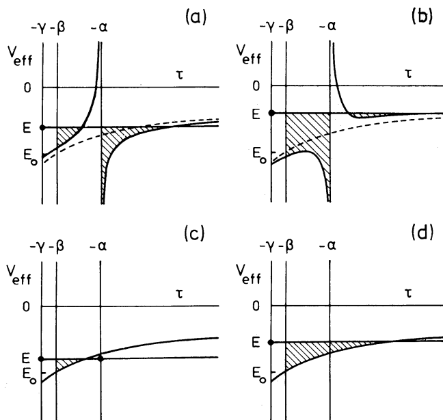
Figure 9. Effective potential curves for orbits in the (x, y) -plane of the perfect ellipsoid. (a) Butterfly; (b) loop; (c) stable y -axis orbit; (d) unstable y -axis orbit.
