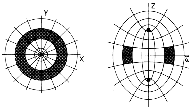
Figure 24. Cross-section with a meridional plane and with the equatorial plane of the volume allowed to a short axis tube by the values of the integrals of motion. The filled circles are the foci.
