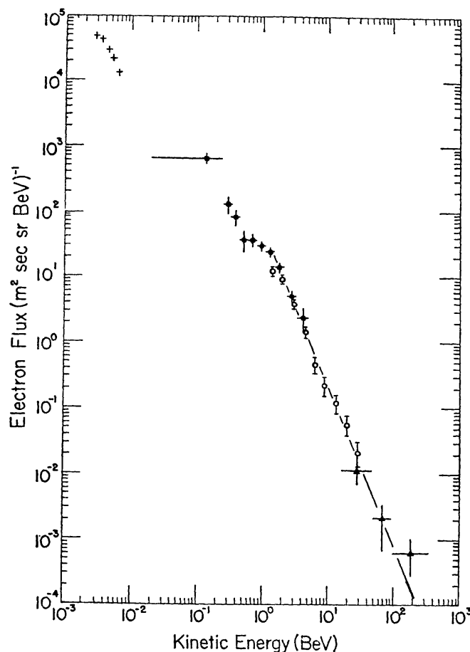
FIG. 1. Energy spectrum of cosmic-ray electrons. This is a composite diagram prepared by Dr. Y. Tanaka (October 1966) from data by Cline et al. (+, 1964), Meyer et al. (●, unpublished), Bleeker et al. (○, unpublished), and Daniel & Stephens (Δ, unpublished).
