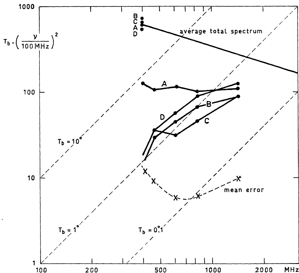
FIG. 2. Spectra of polarized and unpolarized radiation in four regions of the sky (rough sketch based on unpublished data by Brouw). Region A: l=140^\circ , b=5^\circ ; Region B: l=125^\circ , b=5^\circ ; Region C: l=30^\circ , b=30^\circ ; Region D: l=30^\circ , b=50^\circ .
