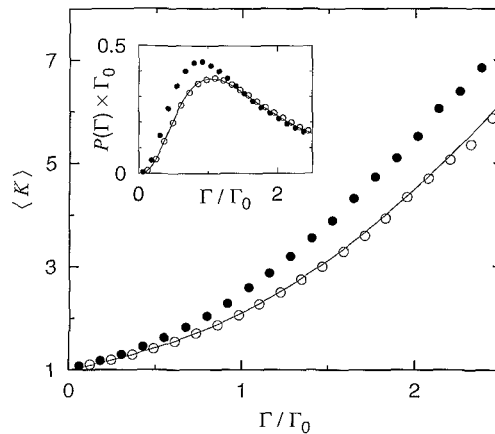
Fig. 9. Average Petermann factor \langle K \rangle for N = 4 , \beta = 2 [open circles: result of a numerical simulation, curve Eq. (4.10)] and for N = 8 , \beta = 1 (filled circles: result of a numerical simulation). The parameter \Gamma_0 equals N\Delta/2\pi in both cases, so it is twice as large for \beta = 2 as for \beta = 1 . The inset depicts the probability distribution of \Gamma .
