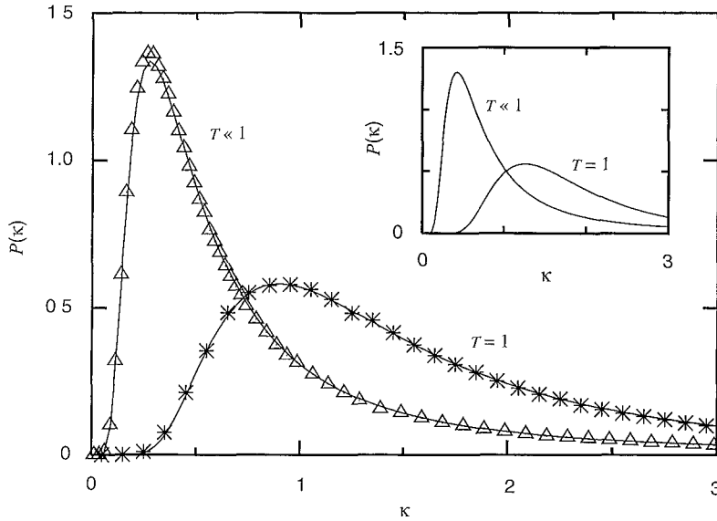
Fig. 2. Probability distribution of the rescaled Petermann factor \kappa = (K - 1)\Delta/TT for T = 1 and T \ll 1 , in the presence of time-reversal symmetry. The solid curves follow from Eqs. (3.20) (with \beta = 1 ) and (3.21a). The data points follow from a numerical simulation of the random-matrix model. The inset shows the results (3.20) (with \beta = 2 ) and (3.21b) for broken time-reversal symmetry.
