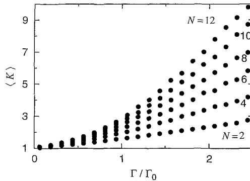
Fig. 8 Results of a numerical simulation of the average Petermann factor \langle K \rangle in the presence of time-reversal symmetry, as a function of the decay rate \Gamma for N fully transmitted scattering channels
