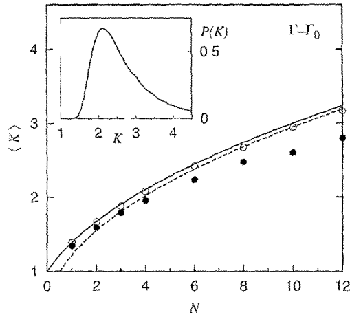
Fig. 6. Average of the Petermann factor K at \Gamma = \Gamma_0 as function of the number N of fully transmitted scattering channels. The analytical result (4.10) for broken time reversal symmetry (full curve) is compared with the result of a numerical simulation (open circles for broken time reversal symmetry; filled circles for preserved time reversal symmetry). The dashed line is the large N result (4.14). The inset shows the distribution of K at \Gamma = \Gamma_0 for N = 10 .
