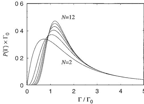
Fig. 4. Decay rate distribution P(\Gamma) of a chaotic cavity with an opening that supports N=2, 4, 6, 8, 10, 12 fully transmitted scattering channels. Computed from Eq. (4.2) for the case of broken time reversal symmetry.
