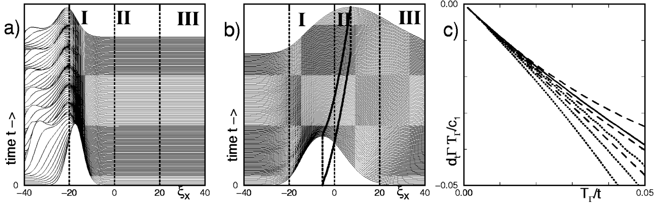
FIG. 2. (a) and (b) Simulation of the QCGL equation as in Fig. 1(b) for times t=35 to 144 . (a) shows |N| (16) as a function of \xi_X . (b) shows |\psi| , which in region I builds up a linear slope \psi \propto \xi_X , and in region III decays like a Gaussian widening in time. The lines in region II show the maxima of \psi(\xi_X, t) for fixed t and their projection \xi_X \sim \sqrt{t} into the (\xi_X, t) plane. (c) shows the scaling plot for the phase relaxation. From left to right: SH (dashed lines) for u = \sqrt{\epsilon} , 0.01\sqrt{\epsilon} , and 0.0001\sqrt{\epsilon} ( \epsilon=5 ), and QCGL (dotted lines) for |A|=0.002 , 0.0002 , and 0.00002 . Plotted is \Gamma(t)T_\Gamma/c_1 vs 1/\tau . Here \tau = t/T_\Gamma , and T_\Gamma = T_v[1 + \lambda^* \text{Im} D^{-1/2}/(q^* \text{Re} D^{-1/2})] . The solid line again is the universal asymptote -1/\tau + 1/\tau^{3/2} .
