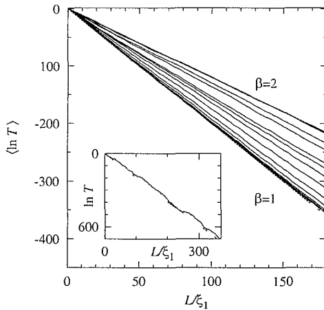
FIG 1 Average logarithmic transmittance \langle \ln T \rangle as a function of wire length L for the Anderson model with N = 5 propagating modes. The two dashed lines have the slopes predicted for preserved ( \beta = 1 ) and broken ( \beta = 2 ) time-reversal symmetry. From bottom to top the data correspond to fluxes \Phi_\xi/\Phi_0 = 0, 0.0005, 0.005, 0.05 (four indistinguishable solid curves), 0.5, 1, 2.5, 5, 10, 15, 20, 25, 40, 50, 75, 125 (two indistinguishable solid curves). The inset shows \ln T for an individual realization with \Phi_\xi = \frac{1}{2} \Phi_0 (solid curve) and the slope of the ensemble-averaged result (dashed line). The statistical error is of the order of the wiggles of the curves.
