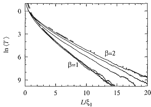
FIG 4 Logarithm of the average transmittance \ln\langle T \rangle as a function of wire length L for the N = 5 Anderson model at various values of the magnetic field (solid curves, from bottom to top, \Phi_\xi/\Phi_0 = 0, 5, 25, 50, 125 ). The dashed curves are the theoretical prediction of Refs [13,14] for zero and large magnetic field
