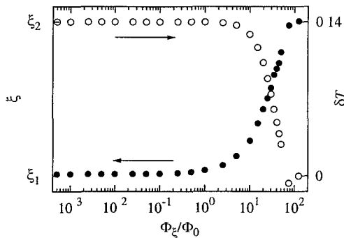
FIG 2 Asymptotic decay length (solid circles) and weak-localization correction \delta T (open circles) as a function of flux for the N = 5 Anderson model. The statistical error is of the order of the size of the circles.
