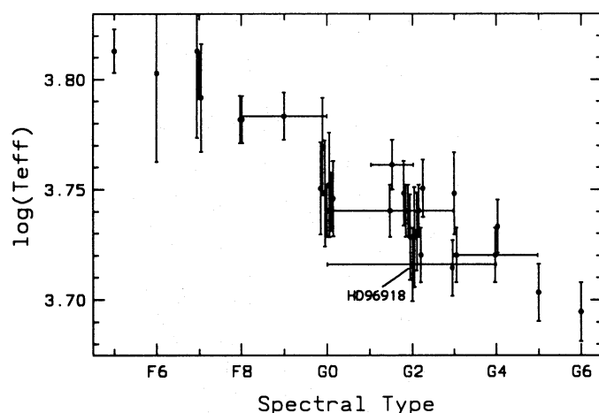
Fig. 6. T_{\text{eff}} vs. spectral type for stars studied here
