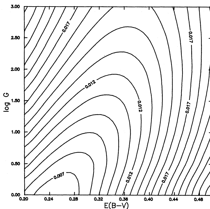
Fig. 1. Contours of \chi -values which represent the fitting quality between the observed and theoretical fluxes for several combinations of \log g and E(B-V) . These contours are calculated for T_{\text{eff}} = 5250 K
