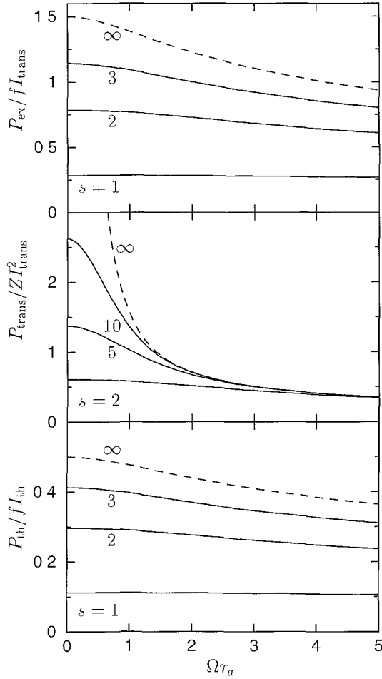
Fig. 3. Frequency dependence of the three super-Poissonian contributions to the noise power, P - \bar{I} = P_{th} + P_{trans} + P_{ex} , for different values of s = L/\xi_a in an absorbing waveguide. The solid curves are computed from equations (3.6–3.8), the dashed curves are the large- s asymptotes (3.10–3.12). The parameter Z is defined as Z = (c\xi_a/2D)(2\pi/N\delta\omega) .
