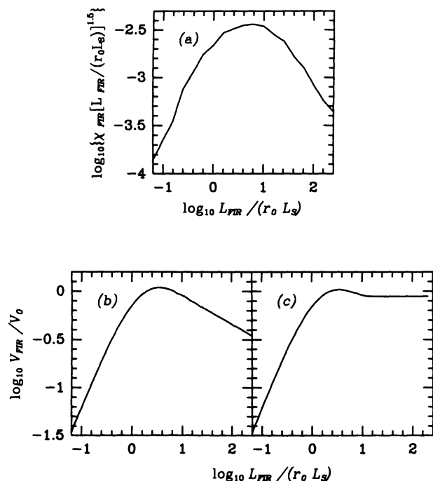
FIG. 6.—(a) Dependence of the observed visibility function V_{FIR} on L_{FIR}/(r_0 L_S) ; see eq. (9). Data for \chi_{FIR} are from Saunders et al. (1990) (see text for more details). In (b) and (c) we show the theoretical ratio between the FIR visibility function V_{FIR} and the constant V_0 as defined in eq. (11). In (b) we have n_* = 1.8 ( \log_{10} r_{sw} = -0.1 ), and in (c) n_* = 1.5 ( \log_{10} r_{sw} = 0.1 ).
