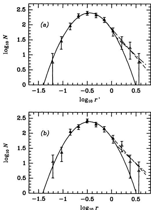
FIG. 3.—Triangles show the distribution of the logarithm of the number of galaxies N in the combined Rb, Rf, and Vo sample, for intervals (a) in d \log_{10} r' and (b) in d \log_{10} r . The solid curve is a Gaussian fit to all the points marked as filled triangles. The dashed line matches the parabolic fit and its derivative at \log_{10} r' = -0.1 in (a) and at \log_{10} r = -0.1 in (b), and is a good fit to the last three points (open triangles to the right). The dash-dot line has a slope of -1.5 and matches the fit at \log_{10} r' = 0.1 in (a) and at \log_{10} r = 0.1 in (b). Error bars denote the N^{0.5} uncertainties.
