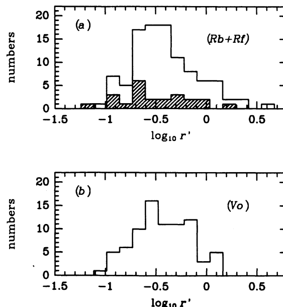
FIG. 2.—(a) Histograms of the logarithm of the ratio r' \equiv r(L_B/L_*)^{-\delta} for galaxies in the Rb + Rf sample. The hatched part of the histogram is for the Rf sample alone. (b) Histograms of the logarithm of the ratio r' for galaxies in the Vo sample.
