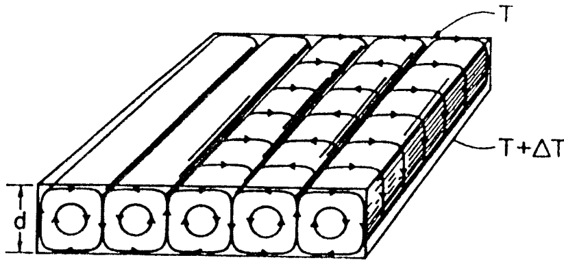
Figure 2: Sketch of parallel convecting rolls in a Rayleigh-Bénard experiment.
