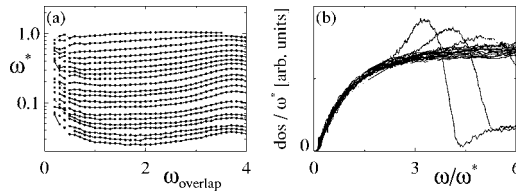
FIG. 2. (a) \omega^* for \mu=10 as a function of \omega_{\text{overlap}} —the regime ( 1 < \omega_{\text{overlap}} < 3 ) corresponds to the crossover regime in the DOS that we focus on here [see text and (b)]. (b) The rescaled DOS for \mu=10 exhibit good data collapse in the crossover regime. Here 20 rescaled DOS are shown with p ranging from 9 \times 10^{-7} to 3 \times 10^{-2} .
