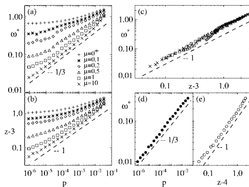
FIG. 3. (a) \omega^* as a function of pressure p for a range of friction coefficients \mu —error bars are similar to or smaller than symbol sizes. (b) Deviation from isotaticity for the same range of parameters. (c) \omega^* scales linearly with the distance to isotaticity for frictional packings. (d), (e) \omega^* for frictionless packings scales with both p and z-4 . Dashed lines indicate power laws with exponents as indicated. For details, see text.
