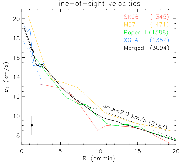
Fig. 3. Velocity dispersion profiles, calculated along concentric rings, for the four different line-of-sight velocity data-sets separately and after they have been merged. The blue dotted curve shows the under-estimated dispersion for the XGEA data-set if also the faint stars are included. From the merged data-set of 3094 stars we select the 2163 stars with line-of-sight velocity errors smaller than 2.0 \text{ km s}^{-1} , resulting in a dispersion profile (black dotted curve) that is not under-estimated due to uncertain line-of-sight velocity measurements.
