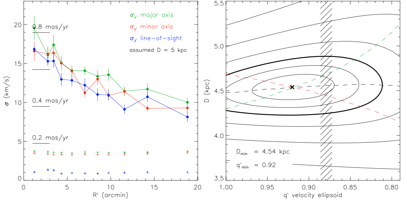
Fig. C.1. Left panel: velocity dispersion profiles calculated along concentric rings. Assuming the canonical distance of 5 kpc, the profiles of the proper motion components in the x' -direction (green) and y' -direction (red) are converted into the same units of \text{km s}^{-1} as the line-of-sight profile in the z' -direction (blue). The black horizontal lines indicate the corresponding scale in \text{mas yr}^{-1} . Below the profiles, the mean velocity error per ring is indicated. Right panel: assuming an oblate velocity ellipsoid with constant (projected) flattening, the ratio of the line-of-sight over the proper motion velocity dispersion profiles yields an estimate for the dynamical distance D . The best-fit values correspond to the minimum (cross) in the \Delta\chi^2 contour plot, where the inner three contours are drawn at the 68.3%, 95.4% and 99.7% (thick contour) levels, and subsequent contours correspond to a factor of two increase in \Delta\chi^2 . For increasing flattening of the velocity ellipsoid, starting with the isotropic case on the left axis, the green (red) dashed curve shows the corresponding best-fit distance if only the profile of the proper motion in the x' -direction ( y' -direction) is used, and the black dashed curve if both are used. The observed flattening from the stellar photometry (Geyer et al. 1983) is indicated by the hashed region.
