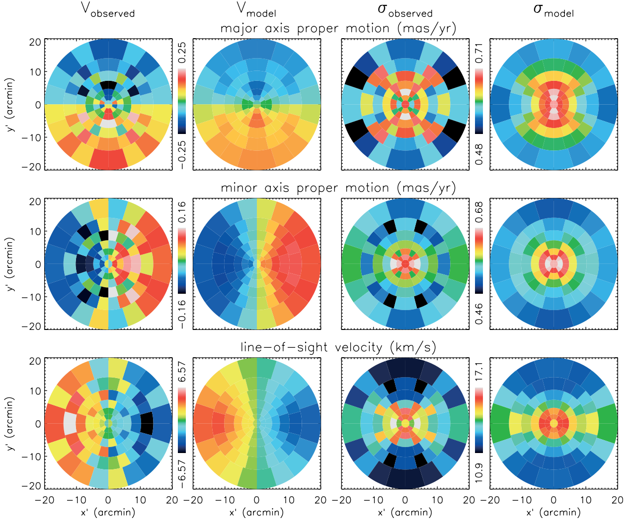
Fig. 9. Mean velocity and velocity dispersion calculated from a power-law model ( first and third column ) and from the best-fit dynamical Schwarzschild model with D = 4.9 kpc, i = 45^\circ and M/L = 2.5 M_\odot/L_\odot ( second and fourth column ). The parameters of the power-law model are chosen such that its observables resemble those of \omega Cen, including the level of noise, which is obtained by randomising the observables according to the uncertainties in the measurements of \omega Cen (see Sect. 6.2 and Appendix B for details). The average proper motion kinematics in the x' -direction ( top row ) and y' -direction ( middle row ), and the average mean line-of-sight kinematics ( bottom row ), calculated in polar apertures in the first quadrant, are unfolded to the other three quadrants to facilitate the visualisation.
