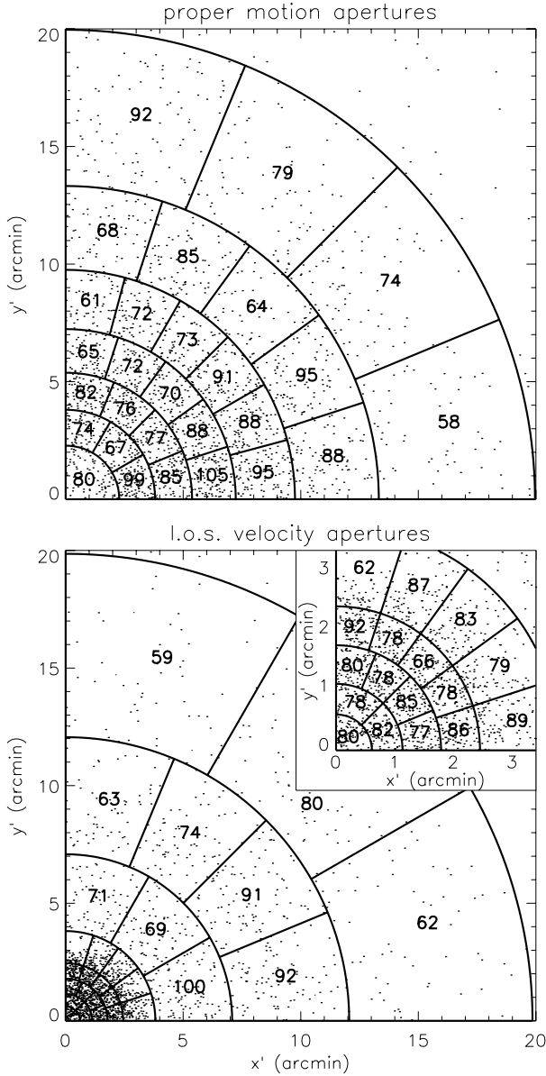
Fig. 13. The polar aperture grid for the proper motions ( top panel ) and for the line-of-sight velocities ( bottom panel ). The dots represent the individual stars, with positions folded to the first quadrant, while the solid lines indicate the locations of the apertures. The number of stars included are indicated in each aperture. An enlargement of the inner part of the line-of-sight polar grid is shown in the top-right corner of the bottom panel.
