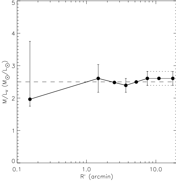
Fig. 16. Variation in mass-to-light ratio M/L_V with projected radius R' . The filled circles represent the eight Gaussian components of the MGE mass model, with the best-fit M/L_V value of each component plotted against its dispersion along the major axis. With the distance and inclination fixed at D = 4.8 kpc and i = 50 degrees, we allowed variation in the M/L_V values for the four inner points with error bar, while the two outer points were shifted vertically similar to the fourth point, and the remaining two points were interpolated between the two neighbouring points. Each of the models was simultaneously fitted to the photometric and kinematic observations of \omega Cen. The error bars represent the 68.3% confidence level for the corresponding \Delta\chi^2 -distribution with four degrees of freedom. The variation in the resulting M/L_V profile is small with no significant deviation from the best-fit constant M/L_V of 2.5 M_\odot/L_\odot (horizontal dashed line).
