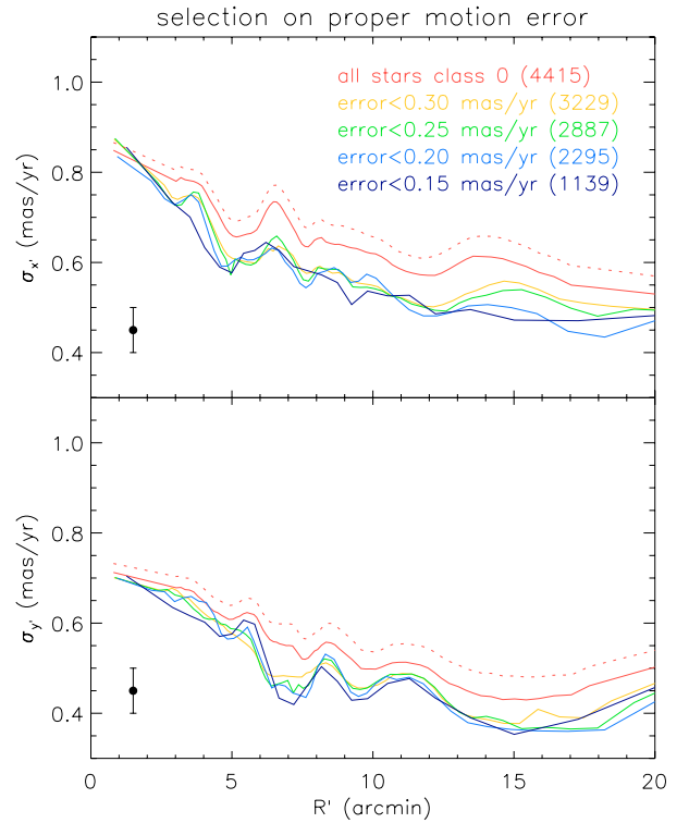
Fig. 2. Proper motion dispersion profiles as in Fig. 1. Starting with all undisturbed (class 0) cluster stars (red solid curve), sequentially a smaller number of stars is selected by setting a tighter limit on the allowed error in their proper motion measurements. The dispersion decreases if the stars with uncertain proper motion measurements are excluded. This effect is significant and larger than the dispersion broadening due to the individual velocity errors, indicated by the red dotted curve. We select the 2295 stars with proper motion error smaller than 0.20 \text{ mas yr}^{-1} , since below this limit the kinematics stay similar.
