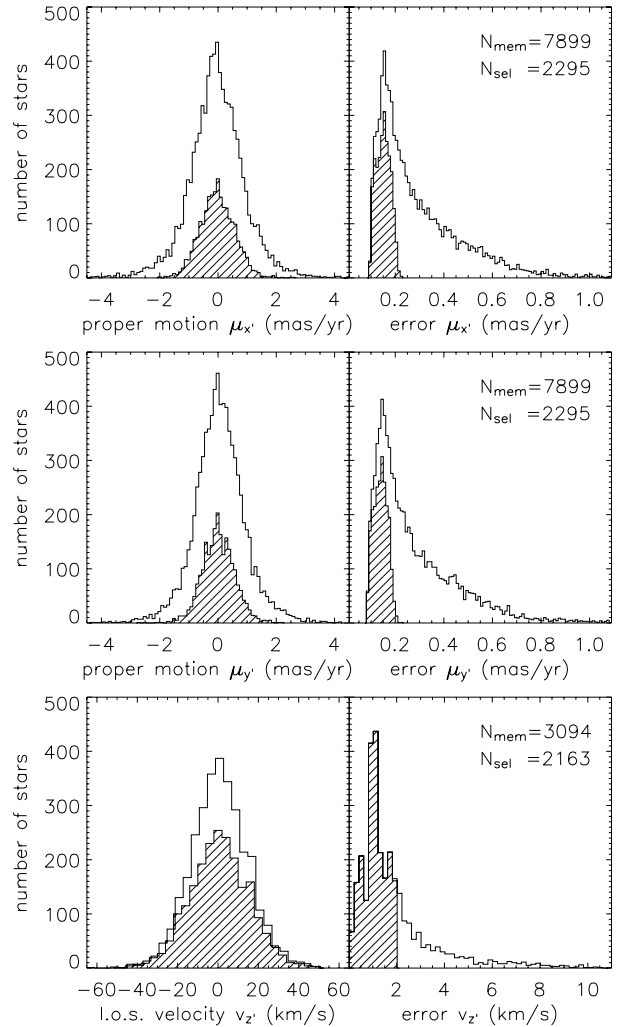
Fig. 5. Histograms of measured velocities ( left panels ) and corresponding velocity errors ( right panels ). The proper motion components \mu_{x'} ( top panels ) and \mu_{y'} ( middle panels ), in the direction of the observed major and minor axis of \omega Cen respectively, come from the photographic plate observations in Paper I. The line-of-sight velocities ( lower panels ) are taken from four different data-sets (Sect. 2.2). The shaded histograms for the N_{\text{sel}} selected stars (Sect. 3) are overlaid on the histograms of the N_{\text{mem}} cluster member stars.
