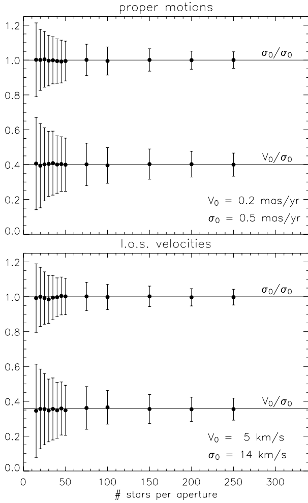
Fig. B.1. Recovery of maximum-likelihood-estimated kinematics from proper motions ( top panel ) and line-of-sight velocities ( bottom panel ). For a given number of stars per aperture, velocities and corresponding errors are simulated by randomly drawing from an intrinsic Gaussian distribution with mean velocity V_0 and velocity dispersion \sigma_0 , broadened by velocity errors randomly drawn from the observed velocity error distributions (left panels Fig. 5). Each filled circle with error bar shows the mean and standard deviation of the measured kinematics from 500 such simulations. As a compromise between lower precision (larger error bars) for a small number of stars per aperture, and lower spatial resolution (larger bins) for a larger number of stars, we choose to have between 50 and 100 stars per bin.
