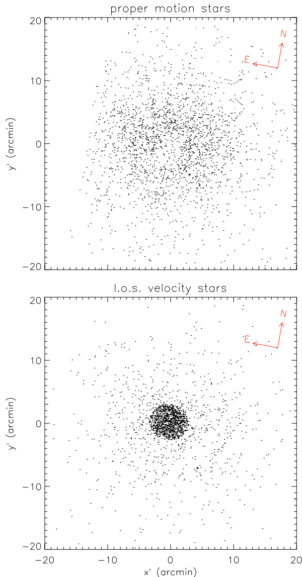
Fig. 4. The stars in \omega Cen with proper motion measurements ( top ) and line-of-sight velocity measurements ( bottom ), that are used in our analysis. The stellar positions are plotted as a function of the projected Cartesian coordinates x' and y' , with the x' -axis aligned with the observed major axis and the y' -axis aligned with the observed minor axis of \omega Cen. The excess of stars with line-of-sight velocities inside the central 3 arcmin in the bottom panel is due to the XGEA data-set.
