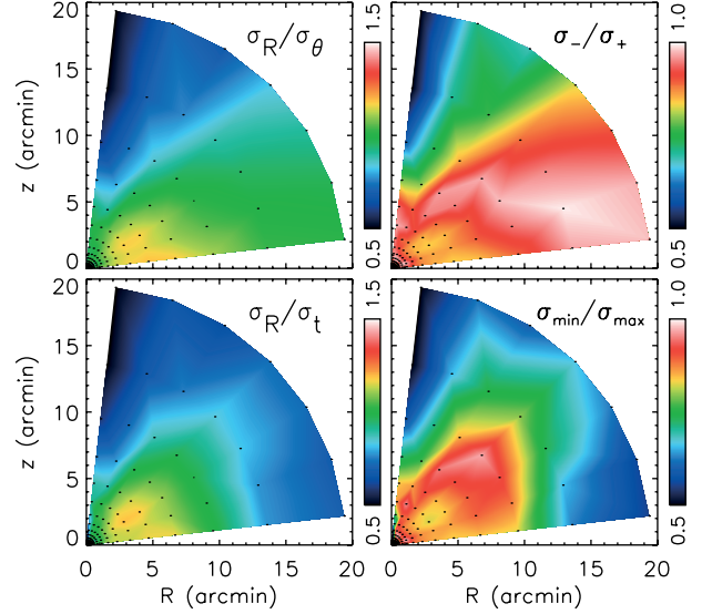
Fig. 18. Degree of anisotropy as function of the equatorial plane radius R and height z (excluding the axes to avoid numerical problems). The top panels show the degree of anisotropy in the meridional plane: left the radial over the angular velocity dispersion and right the minor \sigma_- over the major \sigma_+ semi-axis length of the velocity ellipsoid, taking into account the cross-term \sigma_{R\theta} . The bottom panels include the azimuthal velocity dispersion: left the radial over the tangential velocity dispersion, with \sigma_t^2 = (\sigma_\theta^2 + \sigma_\phi^2)/2 , and right the minimum over the maximum of the three semi-axis lengths \sigma_+ , \sigma_- and \sigma_\phi of the velocity ellipsoid. See text for further details.
