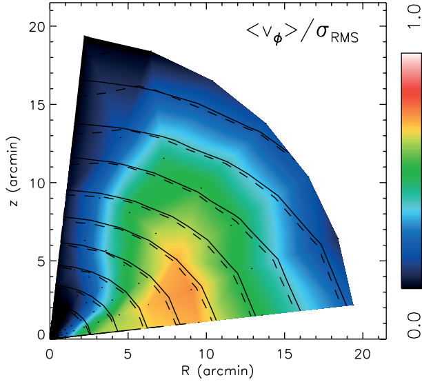
Fig. 17. The colours represent the mean azimuthal rotation \langle v_\phi \rangle in the meridional plane as a function of equatorial plane radius R and height z , and normalised by \sigma_{\text{RMS}} (excluding the axes to avoid numerical problems). The black curves are contours of constant mass density in steps of one magnitude, from the mass model (solid) and from the best-fit model (dashed), showing that the mass is well fitted.
