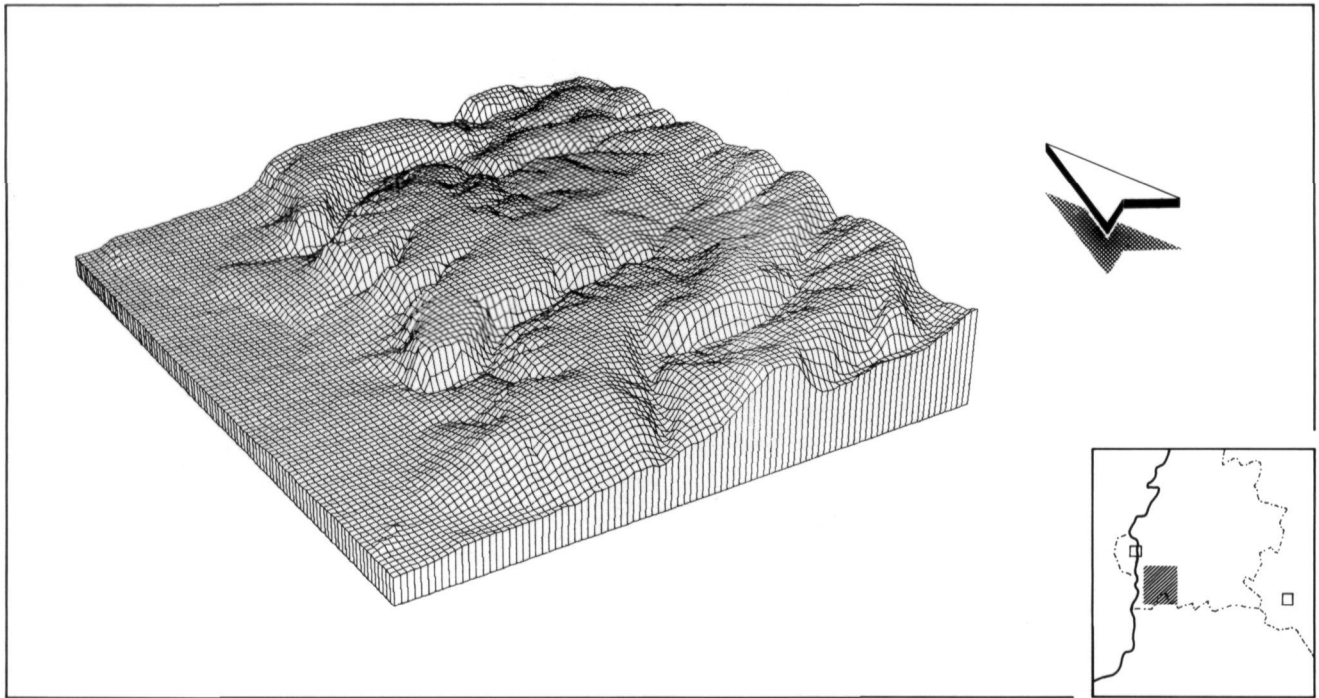
Fig. 11. Three-dimensional view of dry valleys formed in a higher (St.Geertruid) terrace plateau southeast of Maastricht. x between 178000 and 184500, y between 308200 and 315500 in the topographical map system. Vertical scale magnified 8x. Drawing made by -and published with the courtesy of- Dr J. Hartman, Amsterdam.
