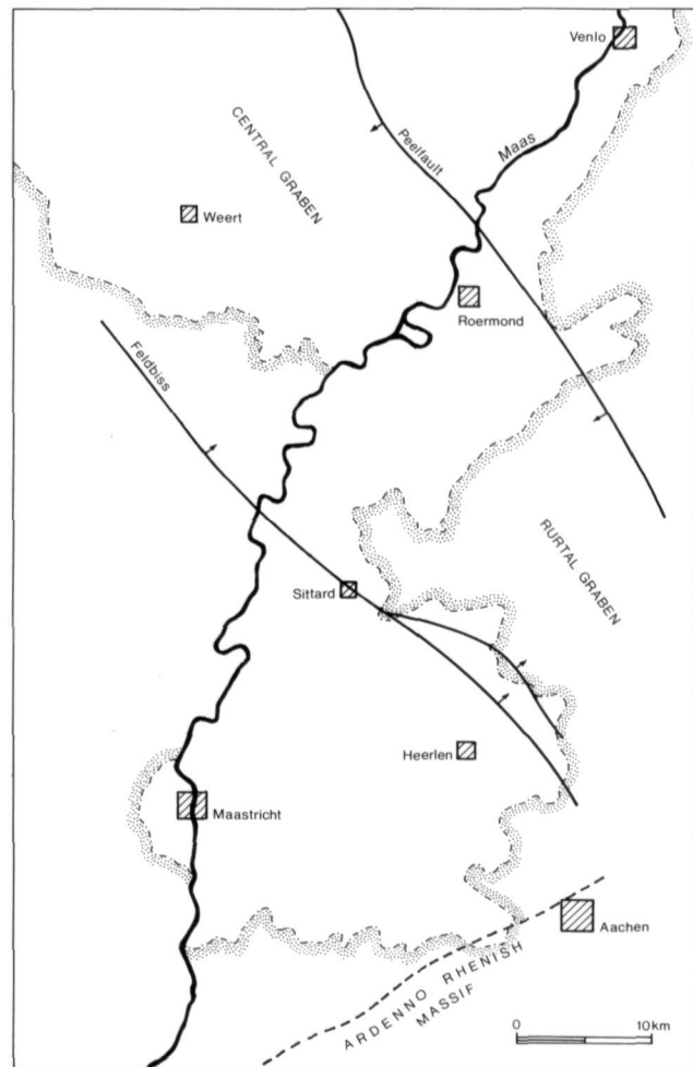
Fig. 7. Structural development of South Limburg (after: Kuyl 1980).
