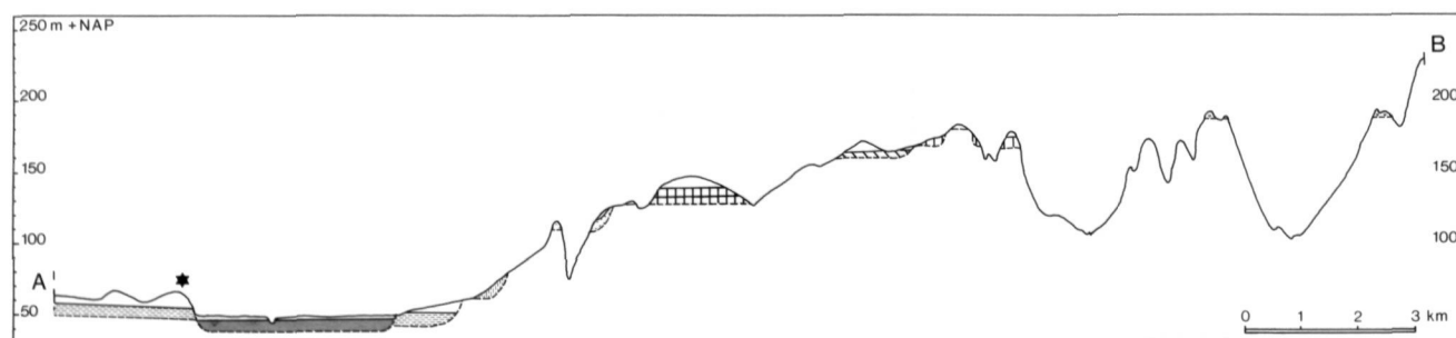
Fig. 9. Cross-section through the terrace landscape of South Limburg, along the A-B line indicated in figure 8. For the symbols used for the terrace bodies see figure 8 (after: Brueren 1945). The position of the Belvédère pit is indicated by an asterisk.
