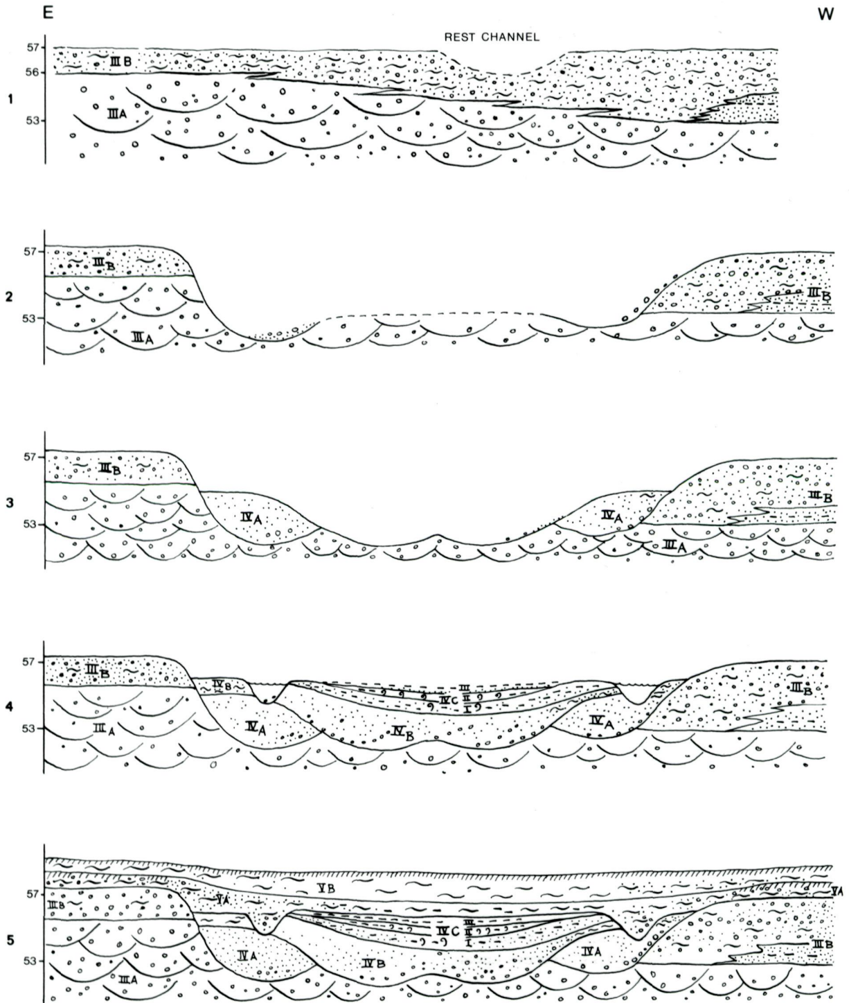
Fig. 19. Idealized representation of the genesis of the Middle Pleistocene sequence at Maastricht-Belvédère. The graphic presentation starts (1) at the end of the braided-river system, the main channel shifting its course to the east of the present Belvédère site. 5 shows the situation after the formation of the Unit V-B deposits (see table 4).
