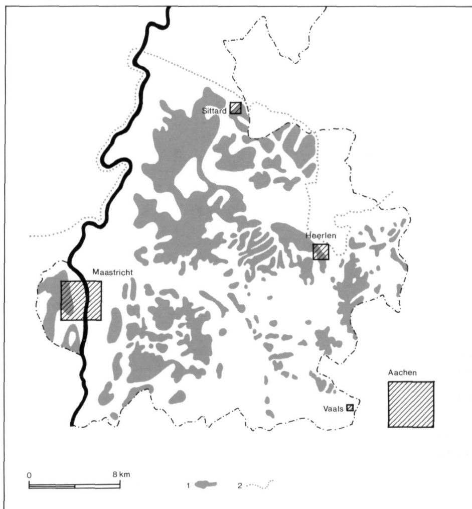
Fig. 10. Distribution of loess layers of over 5 metres thick (1) and the northern boundary of the loess (2) in South Limburg (after: Kuyl 1980).
