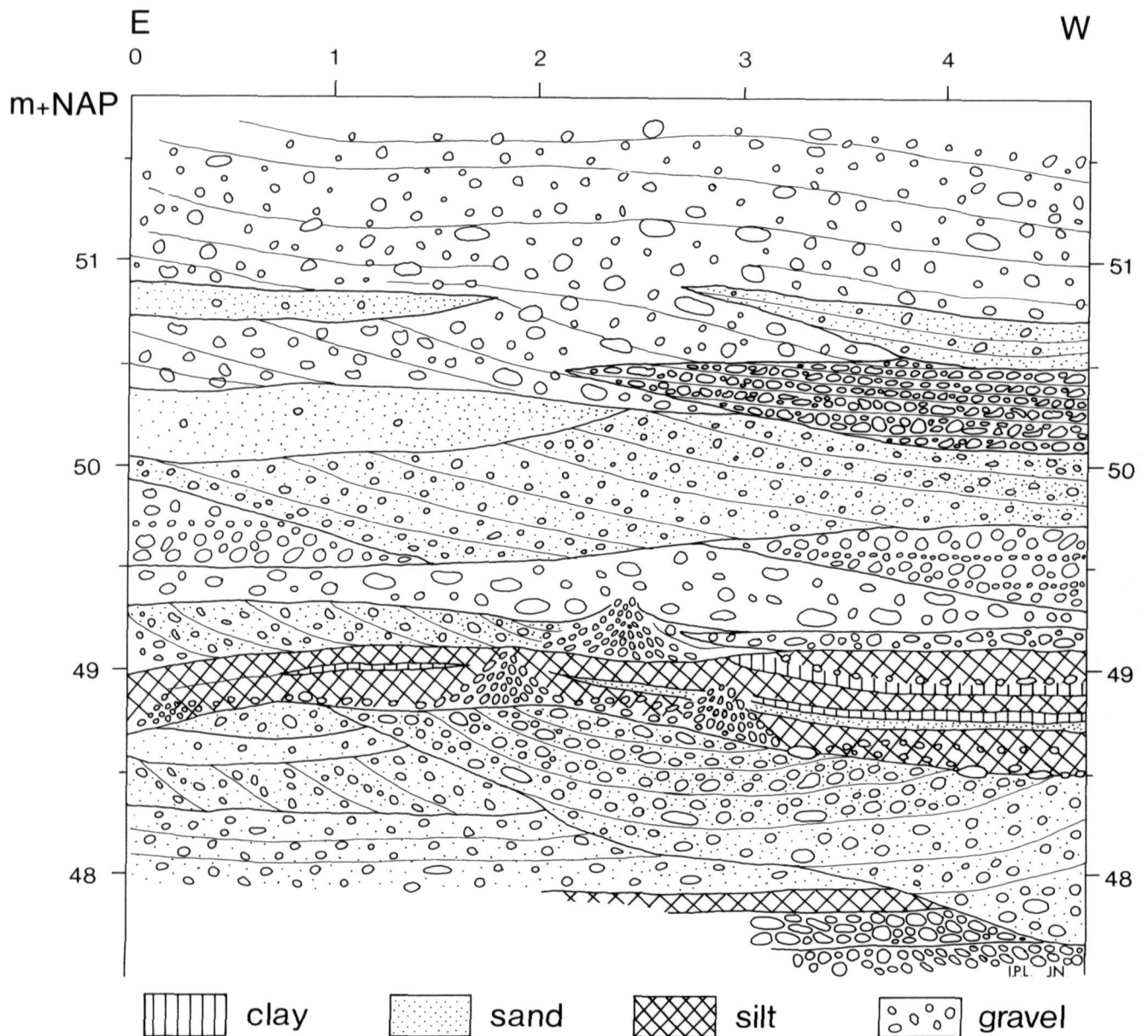
Fig. 12. Representative vertical section through the terrace gravel of Unit 3 (III-A) (from Vandenberghe et al. 1985).
