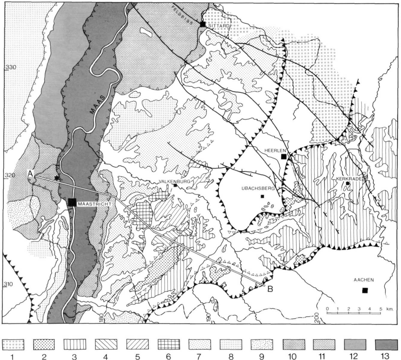
Fig. 8. The Maas terrace geomorphology of South Limburg; drawing based on data provided by the State Geological Survey at Heerlen (pers. comm. P.W. Bosch and W.M. Felder, 1980-1985). The numbers refer to the symbols used for the different terrace bodies: 1=Waubach (Tertiary deposits), 2=Kosberg, 3=Simpelveld, 4=Margraten, 5=Sibbe, 6=Valkenburg, 7=St.Geertruid, 8=St.Pietersberg, 9='s Gravenvoeren, 10=Rothem, 11=Caberg, 12=Eisden-Lanklaar, 13=Oost-Maarland. See also Table 2. (The position of the Belvédère pit is indicated by an asterisk.) The A-B line refers to the cross-section shown in figure 9.
