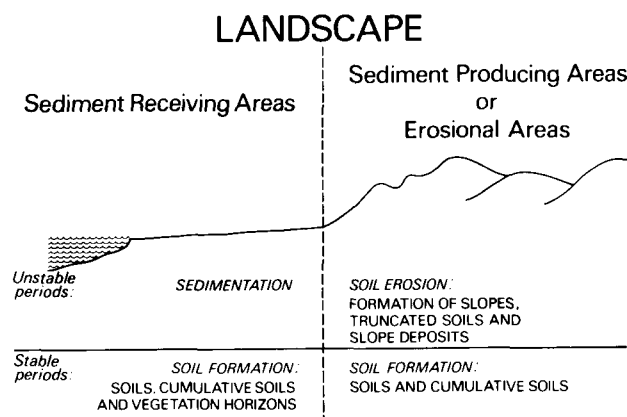
Fig. 16. Schematic representation of the events that take place in the landscape during stable and unstable periods (from Mücher 1985).
