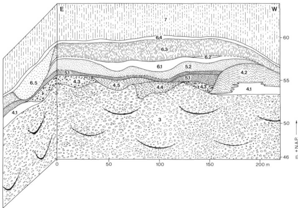
Fig. 14. Schematic cross-section through the Belvédère pit, based on the 1987 fieldwork of the Institute of Earth Sciences, Free University, Amsterdam, showing the stratigraphical position of the lithological units. Vertical scale magnified 12x.
