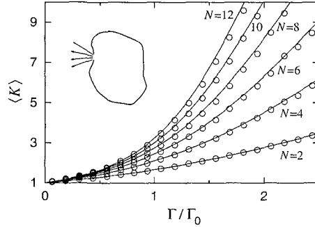
Fig. 1 – Average Petermann factor \langle K \rangle as a function of the decay rate \Gamma (in units of \Gamma_0 = N\Delta/2\pi ) for a chaotic cavity (inset) having an opening which supports N fully transmitted scattering channels. The solid curves are the analytical result (14), the data points are a numerical simulation.
