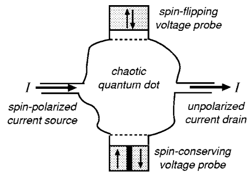
FIG. 1. Illustration of the model. A current I is passed through a quantum dot via two single-channel leads, at a voltage difference V . Spin-flip scattering and decoherence (with relaxation times T_1 and \tau_\phi ) are introduced by means of fictitious voltage probes, separated from the quantum dot by tunnel barriers (dashed lines). The lower (ferromagnetic) voltage probe reinjects an electron into the quantum dot with the same spin but a random phase (contributing only to \tau_\phi ). The upper (normal metal) voltage probe randomizes both spin and phase (contributing to both T_1 and \tau_\phi ).
