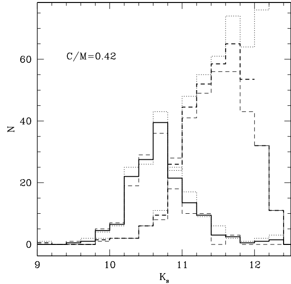
Fig. 3. Distribution of C and M stars as a function of K_s mag in sector N of ring number 3 (Fig. 2). The histogram peaking at about K_s = 10.7 is due to C stars while M stars populate the peak at fainter mag ( K_s = 11.7 ). The dotted line indicates the distribution of stars selected from the 2MASS data while the dashed line indicates the distribution of stars selected from the DCMC data. The thick continuous and dashed lines are the average of both data sets for K_s < 12 while for K_s > 12 the distribution of M stars is strictly that of DCMC data. These thick lines show the final histogram obtained from the observational data that is later compared with a theoretical distribution. The ratio between C and M stars obtained from this final histogram is also indicated.
